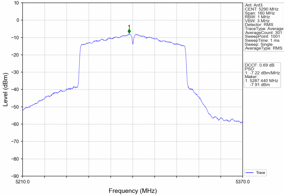
802.11ac(VHT80)_MCH_5290MHz_MIMO_NTNV
