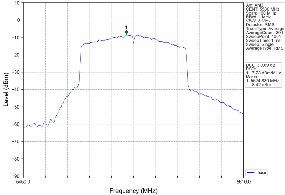
802.11ac(VHT80)_LCH_5530MHz_MIMO_NTNV
