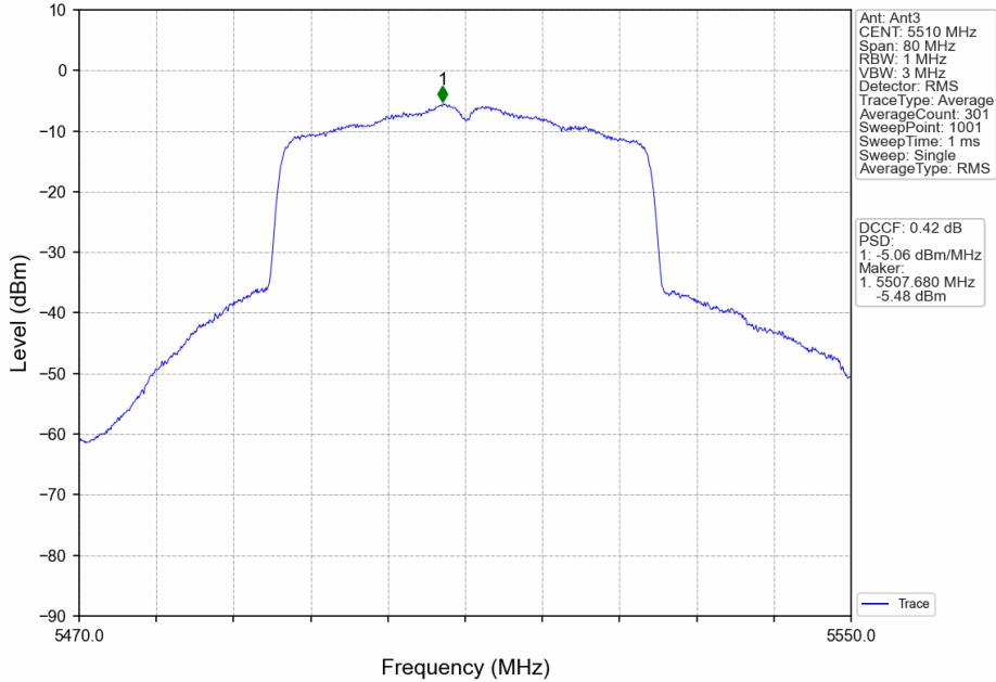
802.11ax(HEW40)_LCH_5510MHz_RU484_Left_MIMO_NTNV
