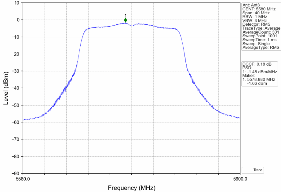
802.11ac(VHT20)_MCH_5580MHz_MIMO_NTNV
