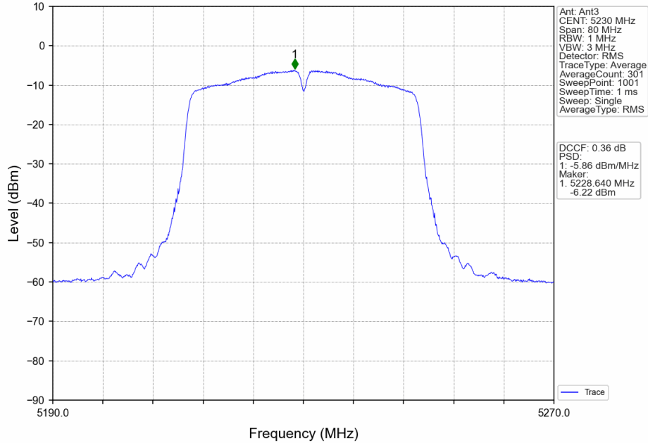
802.11ac(VHT40)_HCH_5230MHz_MIMO_NTNV
