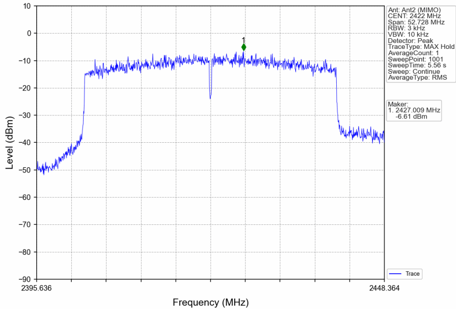
802.11ax(HEW40)_LCH_2422MHz_RU484_Left_MIMO_NTNV
