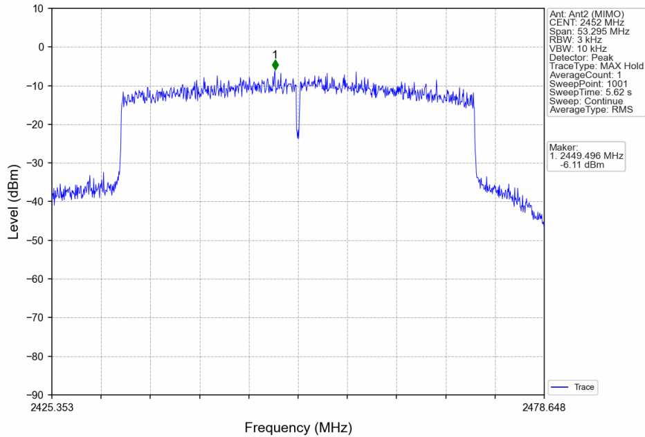
802.11ax(HEW40)_HCH_2452MHz_RU484_Left_MIMO_NTNV
