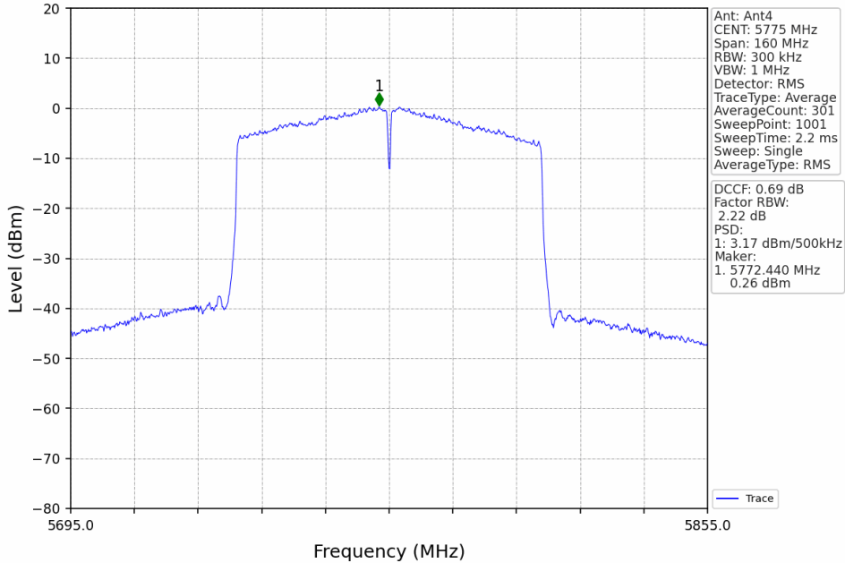
802.11ac(VHT80)_MCH_5775MHz_MIMO_NTNV
