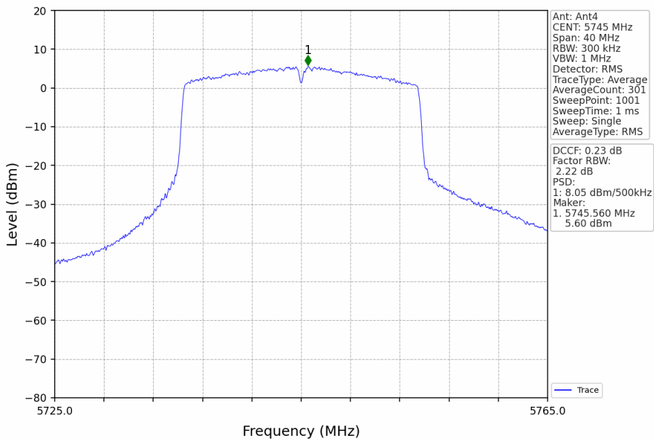
802.11ax(HEW20)_LCH_5745MHz_RU242_Left_Ant4_NTNV
