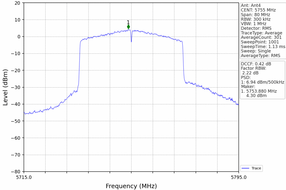
802.11ax(HEW40)_LCH_5755MHz_RU484_Left_MIMO_NTNV
