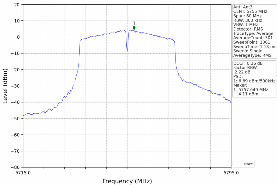
802.11ac(VHT40)_LCH_5755MHz_Ant3_NTNV
