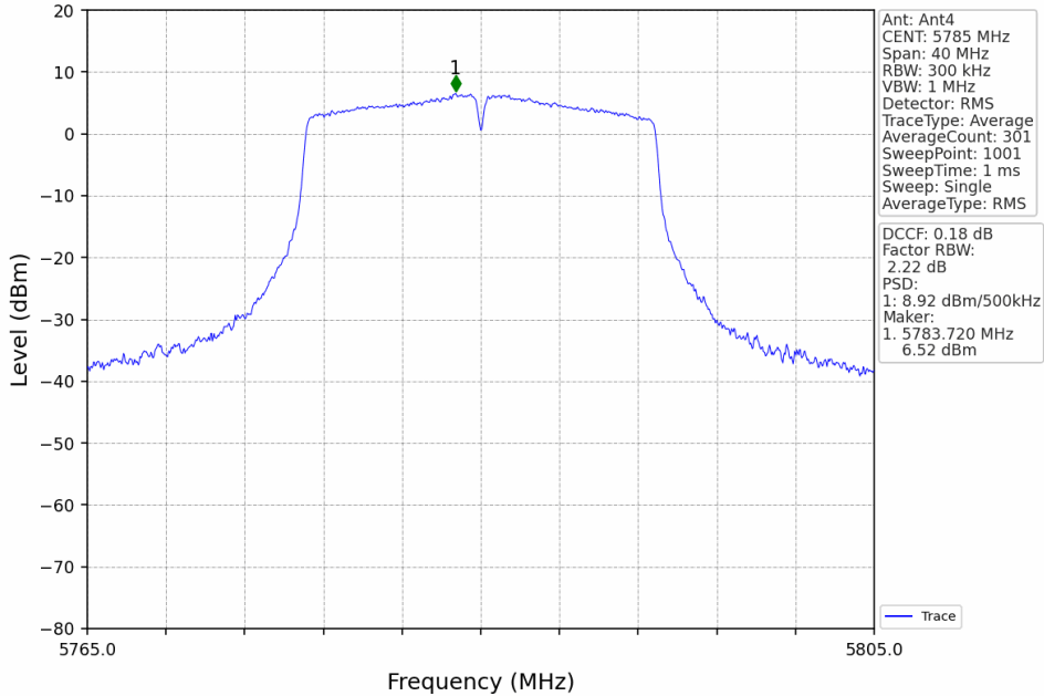
802.11ac(VHT20)_MCH_5785MHz_MIMO_NTNV
