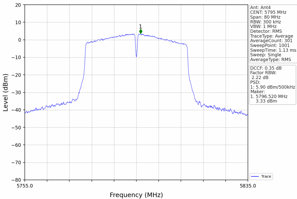
802.11ac(VHT40)_HCH_5795MHz_Ant4_NTNV
