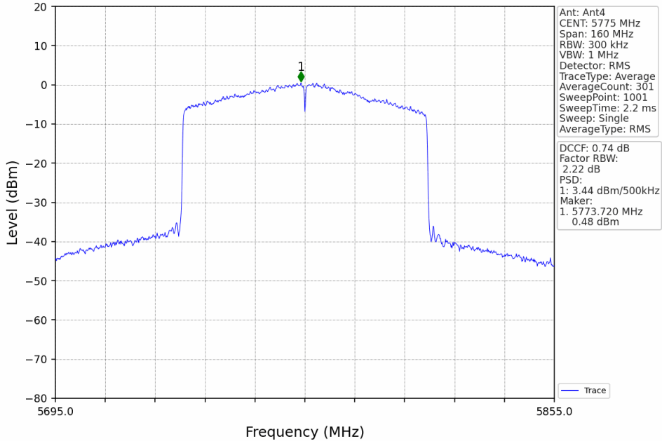
802.11ax(HEW80)_MCH_5775MHz_RU996_Left_MIMO_NTNV
