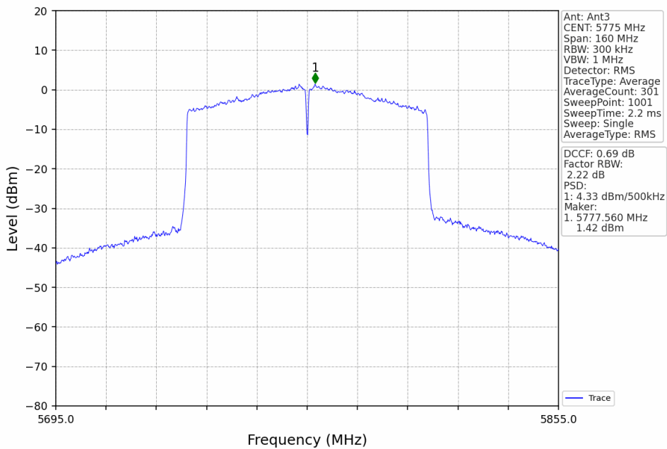
802.11ac(VHT80)_MCH_5775MHz_Ant3_NTNV
