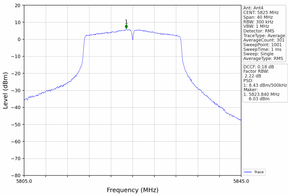
802.11ac(VHT20)_HCH_5825MHz_Ant4_NTNV
