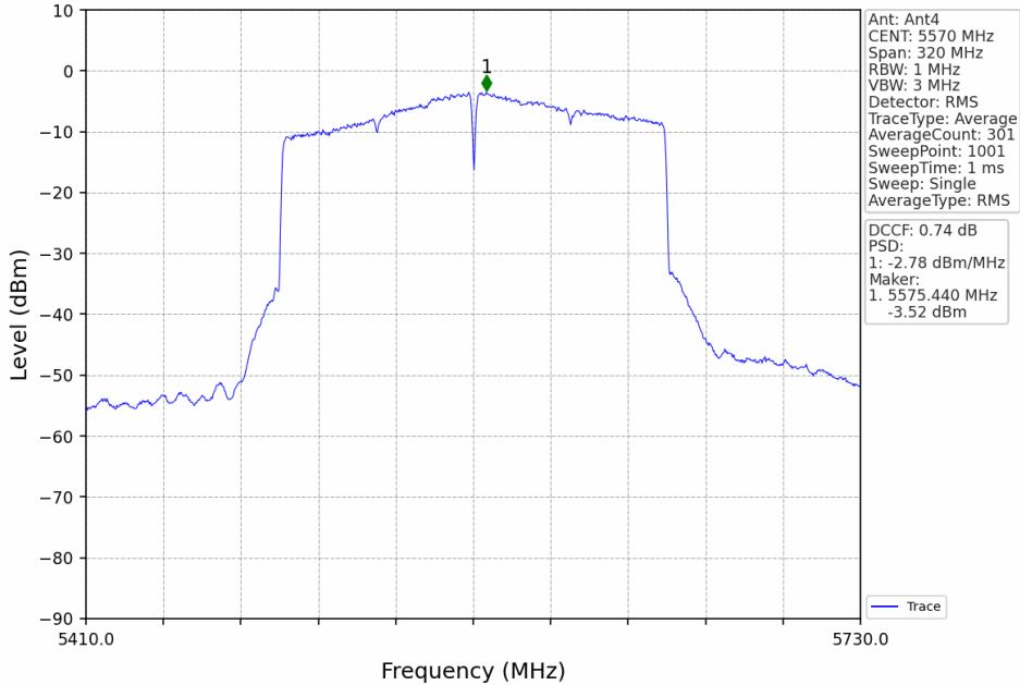
802.11ax(HEW160)_MCH_5570MHz_2xRU996_Left_MIMO_NTNV
