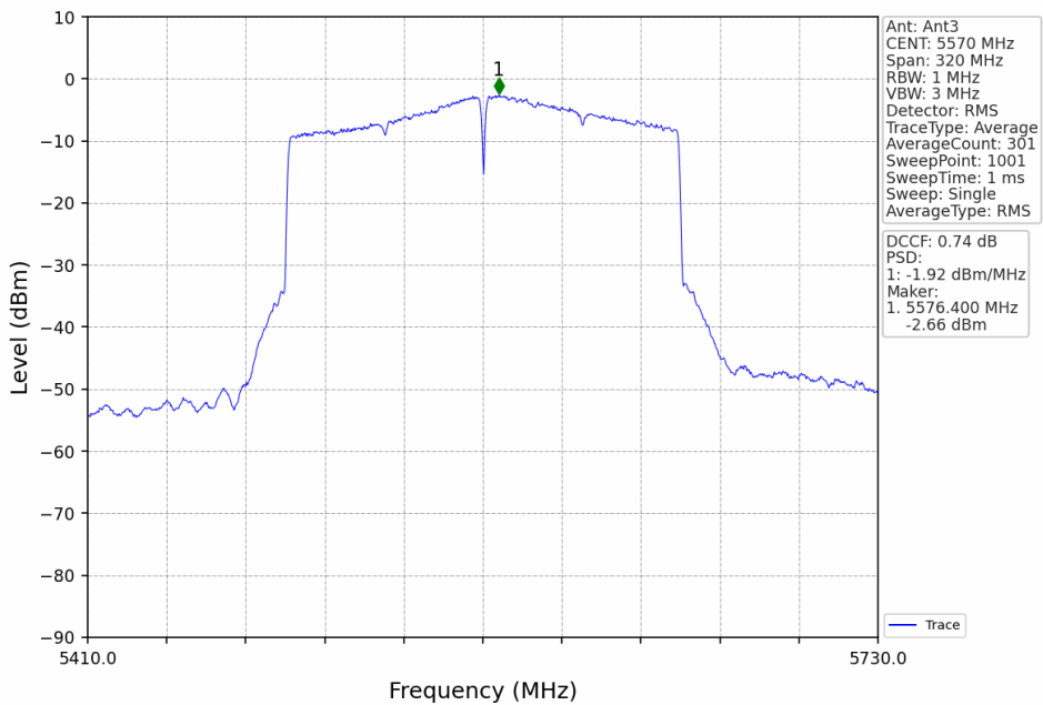
802.11ax(HEW160)_MCH_5570MHz_2xRU996_Left_Ant3_NTNV
