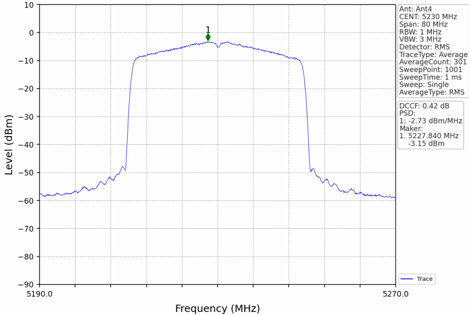
802.11ax(HEW40)_HCH_5230MHz_RU484_Left_MIMO_NTNV
