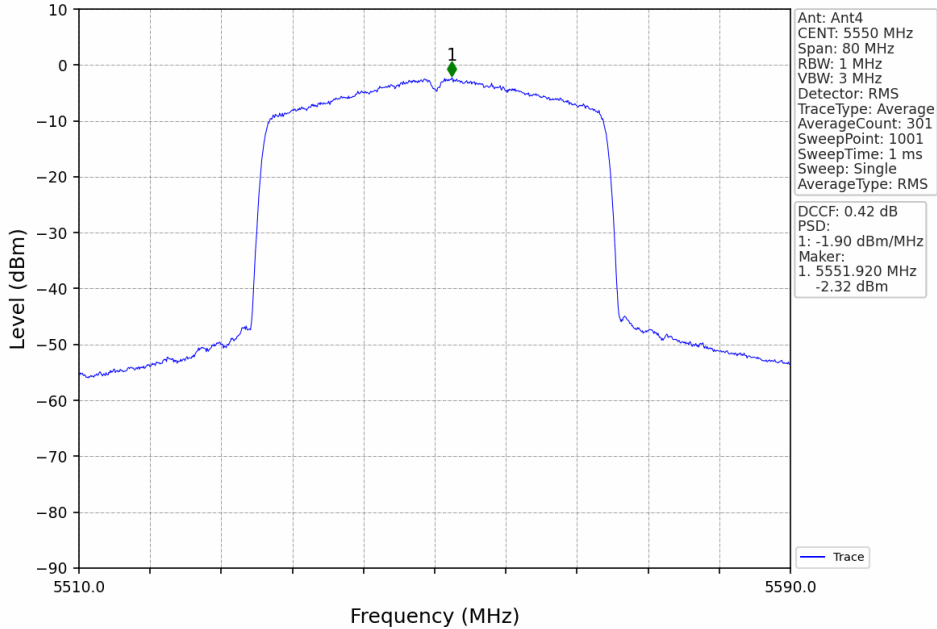
802.11ax(HEW40)_MCH_5550MHz_RU484_Left_MIMO_NTNV
