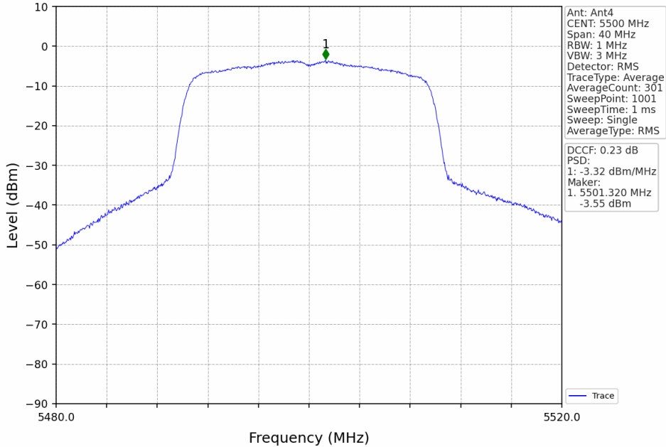
802.11ax(HEW20)_LCH_5500MHz_RU242_Left_MIMO_NTNV
