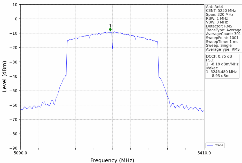
802.11ax(HEW160)_MCH_5250MHz_2xRU996_Left_Ant4_NTNV
