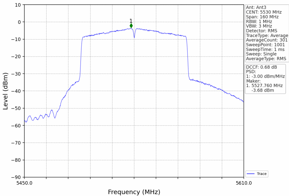
802.11ac(VHT80)_LCH_5530MHz_Ant3_NTNV
