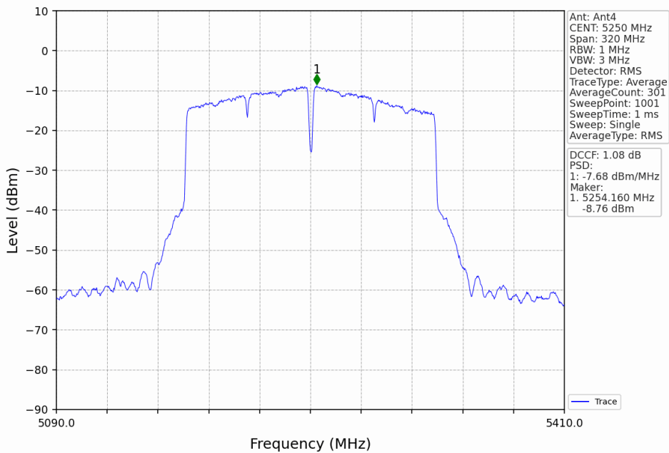
802.11ac(VHT160)_MCH_5250MHz_Ant4_NTNV
