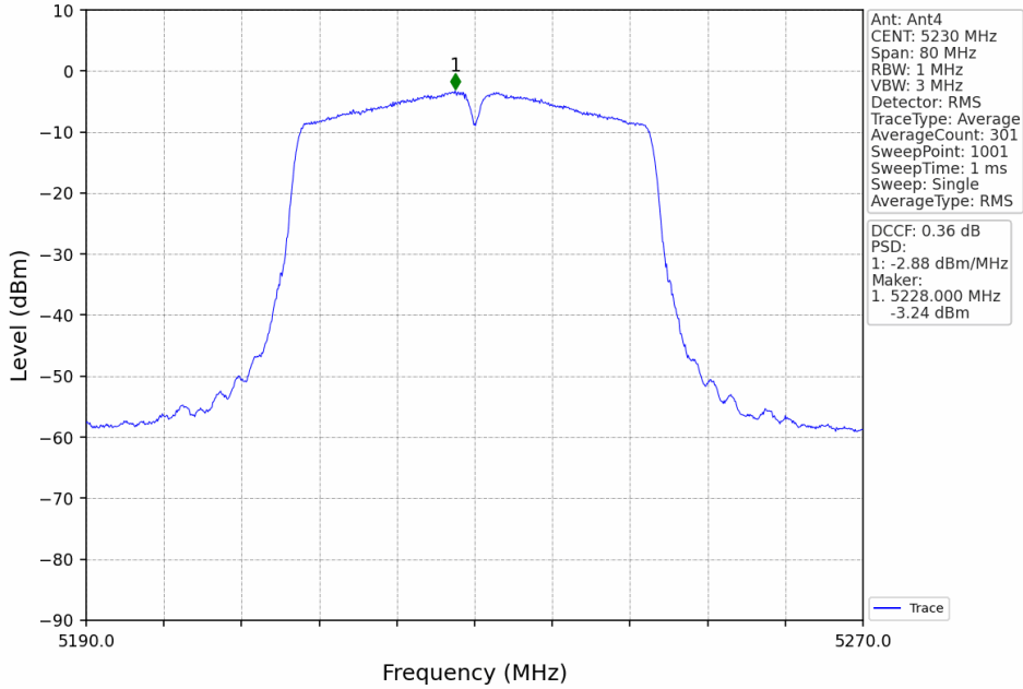
802.11ac(VHT40)_HCH_5230MHz_MIMO_NTNV
