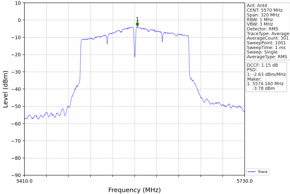
802.11ac(VHT160)_MCH_5570MHz_MIMO_NTNV
