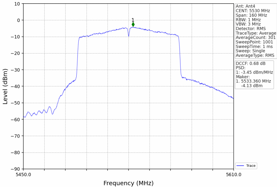
802.11ac(VHT80)_LCH_5530MHz_MIMO_NTNV
