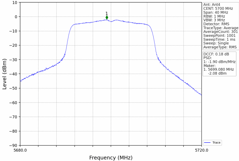
802.11ac(VHT20)_HCH_5700MHz_MIMO_NTNV
