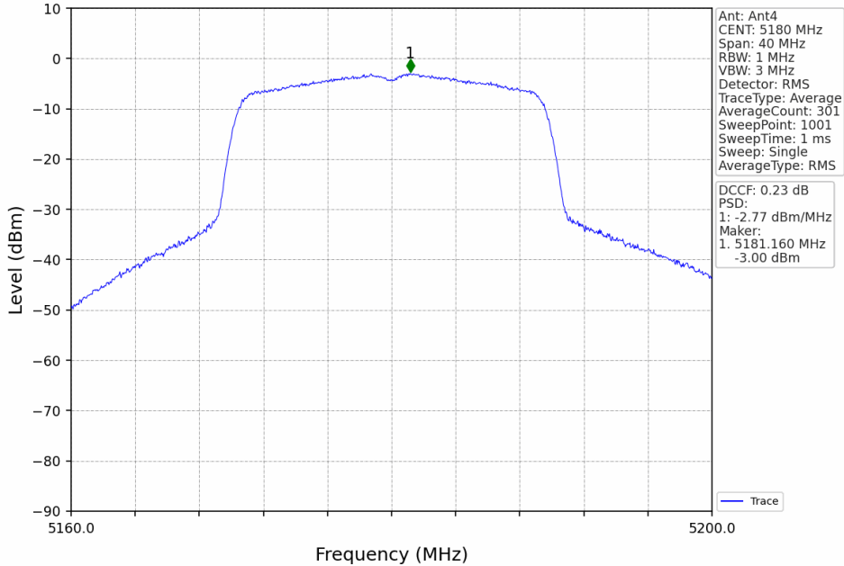
802.11ax(HEW20)_LCH_5180MHz_RU242_Left_MIMO_NTNV
