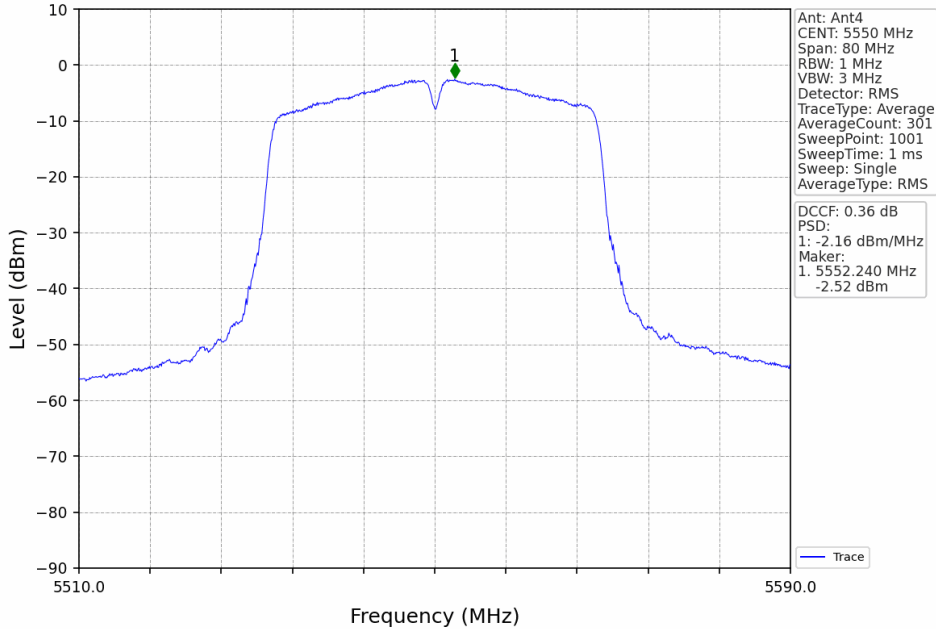
802.11ac(VHT40)_MCH_5550MHz_MIMO_NTNV
