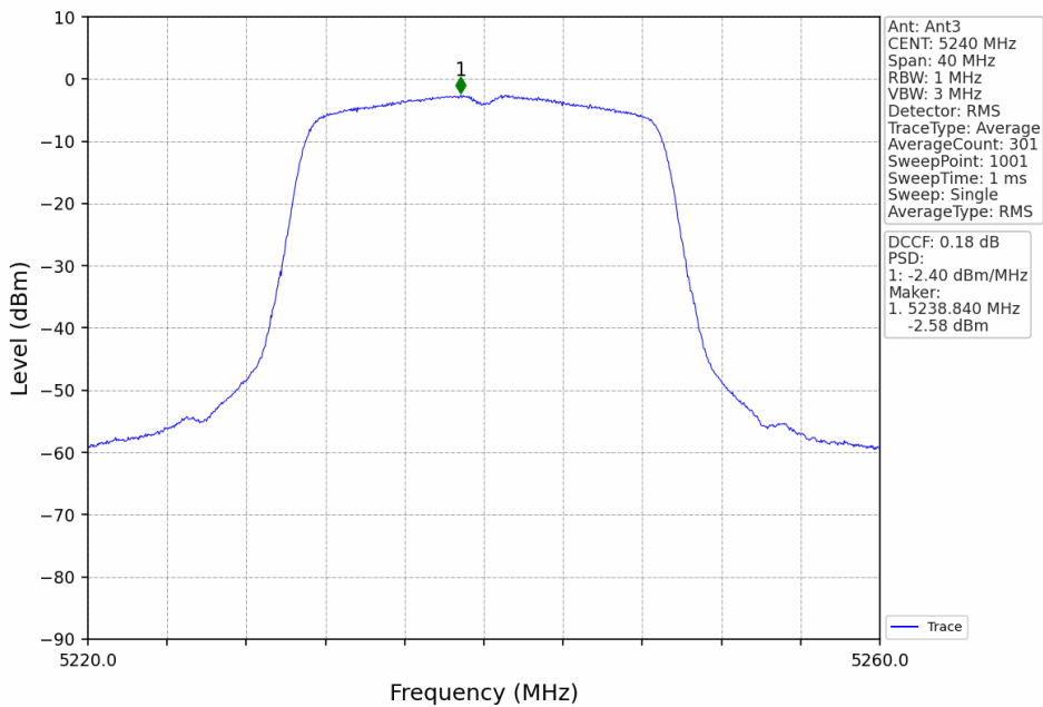
802.11ac(VHT20)_HCH_5240MHz_Ant3_NTNV
