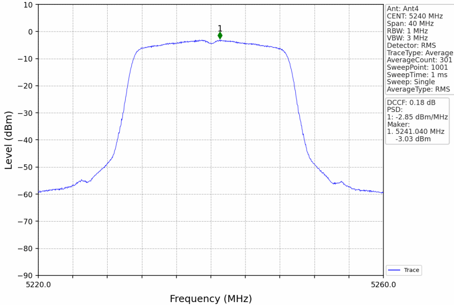
802.11ac(VHT20)_HCH_5240MHz_MIMO_NTNV
