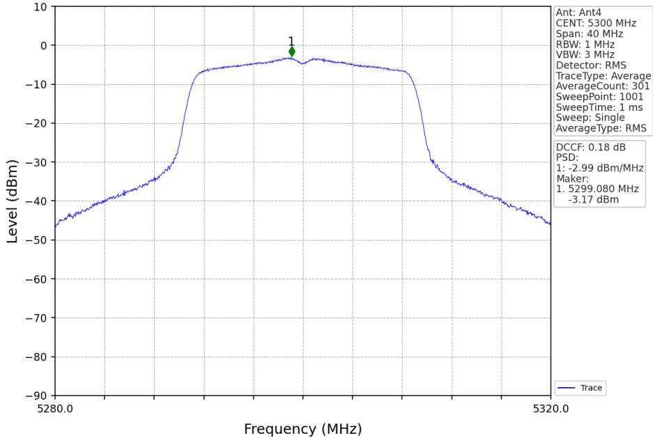
802.11ac(VHT20)_MCH_5300MHz_MIMO_NTNV
