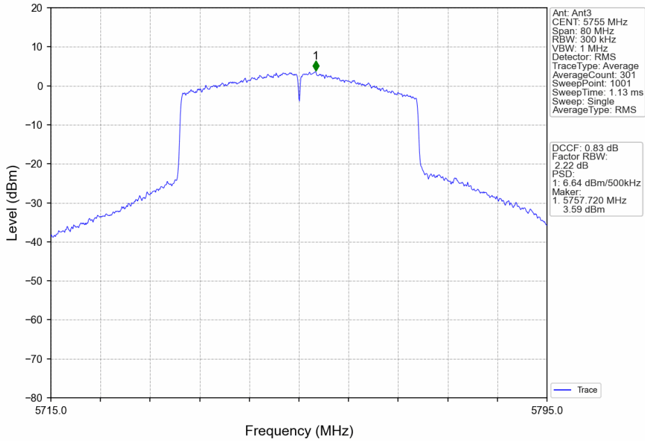
802.11ax(HEW40)_LCH_5755MHz_RU484_Left_MIMO_NTNV
