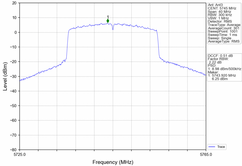
802.11ax(HEW20)_LCH_5745MHz_RU242_Left_MIMO_NTNV
