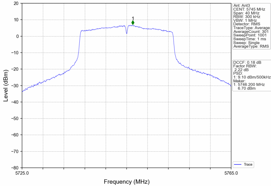
802.11n(HT20)_LCH_5745MHz_MIMO_NTNV
