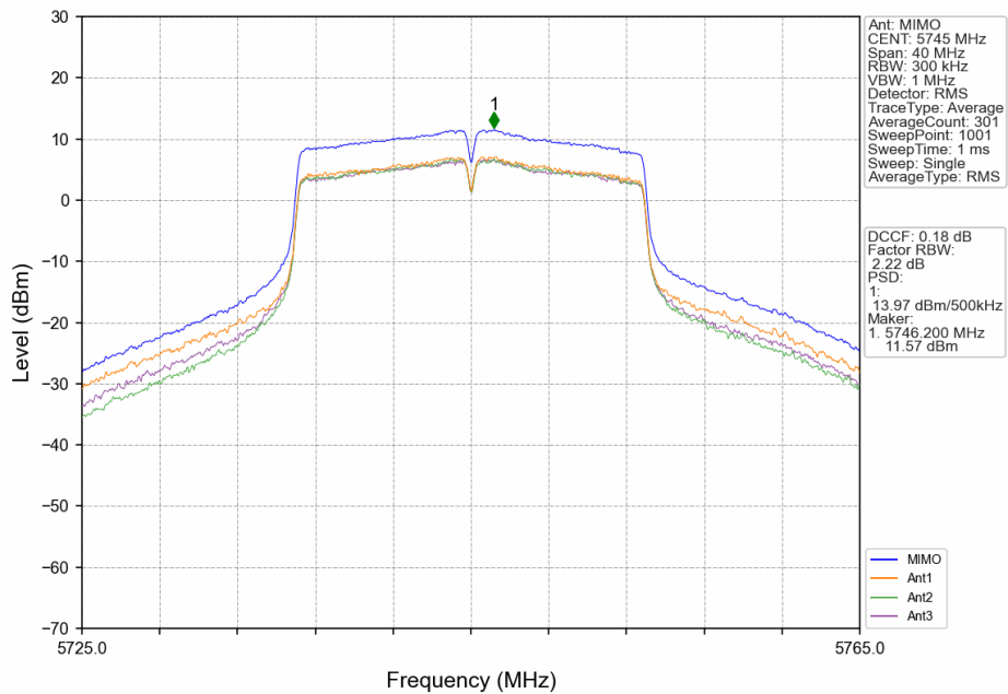
802.11n(HT20)_LCH_5745MHz_MIMO_NTNV
