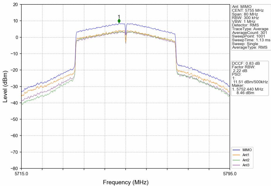
802.11ax(HEW40)_LCH_5755MHz_RU484_Left_MIMO_NTNV
