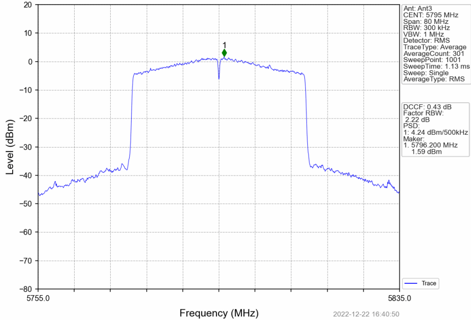
802.11ax(HEW40)_HCH_5795MHz_RU484_Left_MIMO_NTNV
