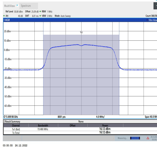
11A-Ant2-5700-TPC L-----15.94-95.89-0.18
