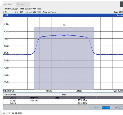
11A-Ant2-5260-TPC L-----15.59-96.55-0.15
