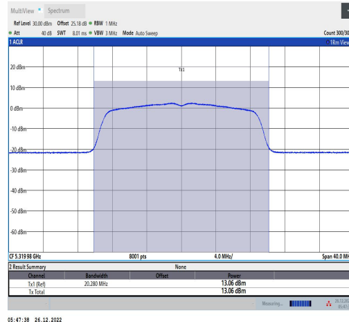
11N20MIMO-Ant1-5320-TPC L-----12.90-96.32-0.16
