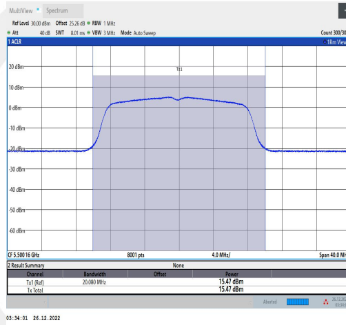
11A-Ant1-5500-TPC L-----15.28-95.67-0.19
