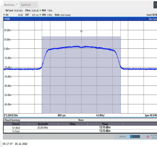
11N20MIMO-Ant1-5260-TPC L-----12.94-96.32-0.16
