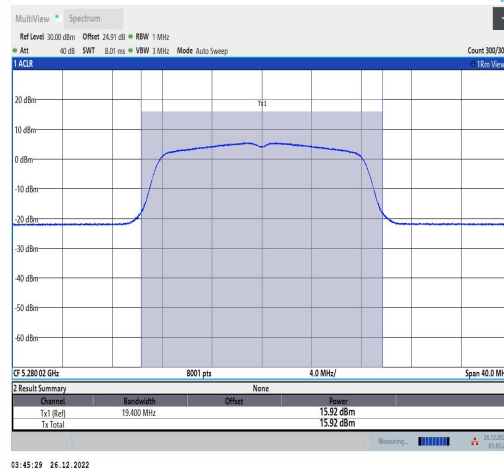
11A-Ant2-5280-TPC L-----15.77-96.55-0.15
