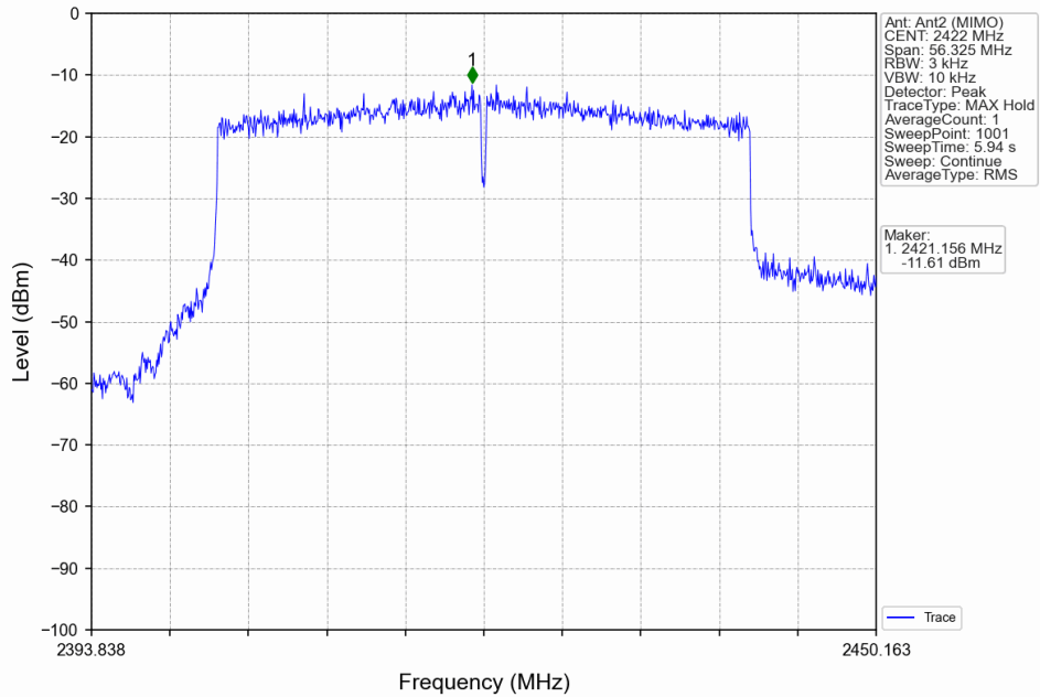
802.11ax(HEW40)_LCH_2422MHz_RU484_Left_MIMO_NTNV
