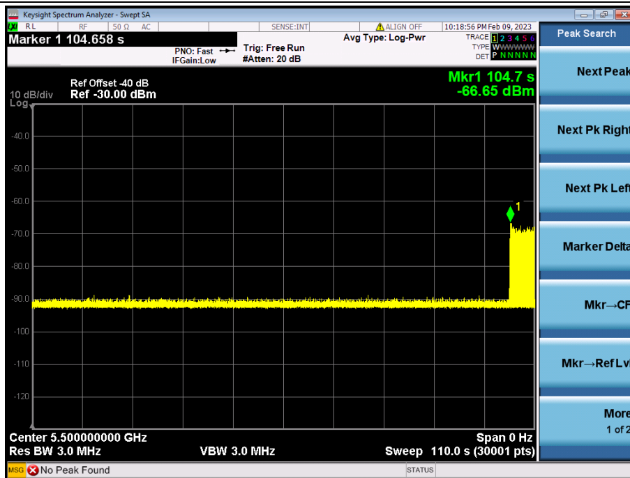
power-on cycle(5500MHz)
