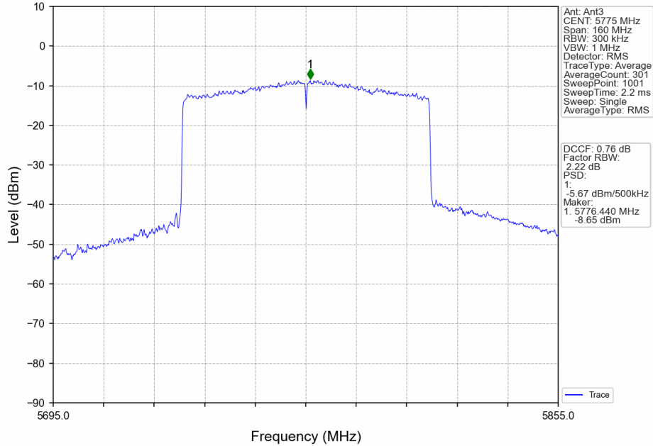
802.11ax(HEW80)_MCH_5775MHz_RU996_Left_MIMO_NTNV
