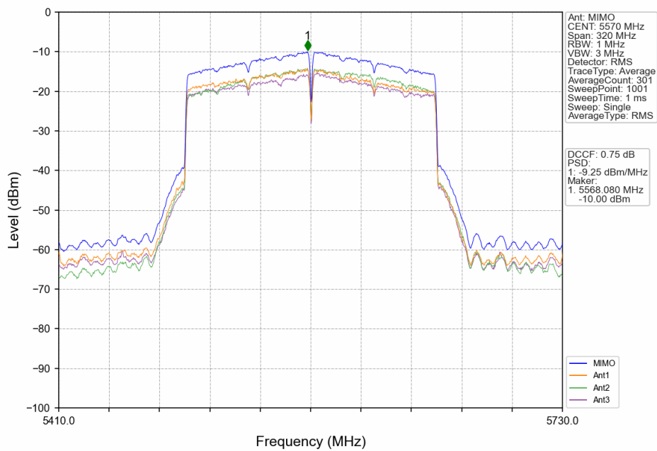
802.11ax(HEW160)_MCH_5570MHz_2xRU996_Left_MIMO_NTNV
