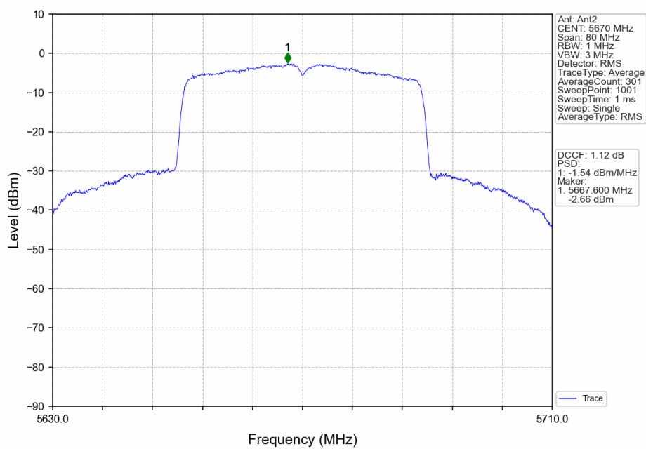
802.11ax(HEW40)_HCH_5670MHz_RU484_Left_Ant2_NTNV
