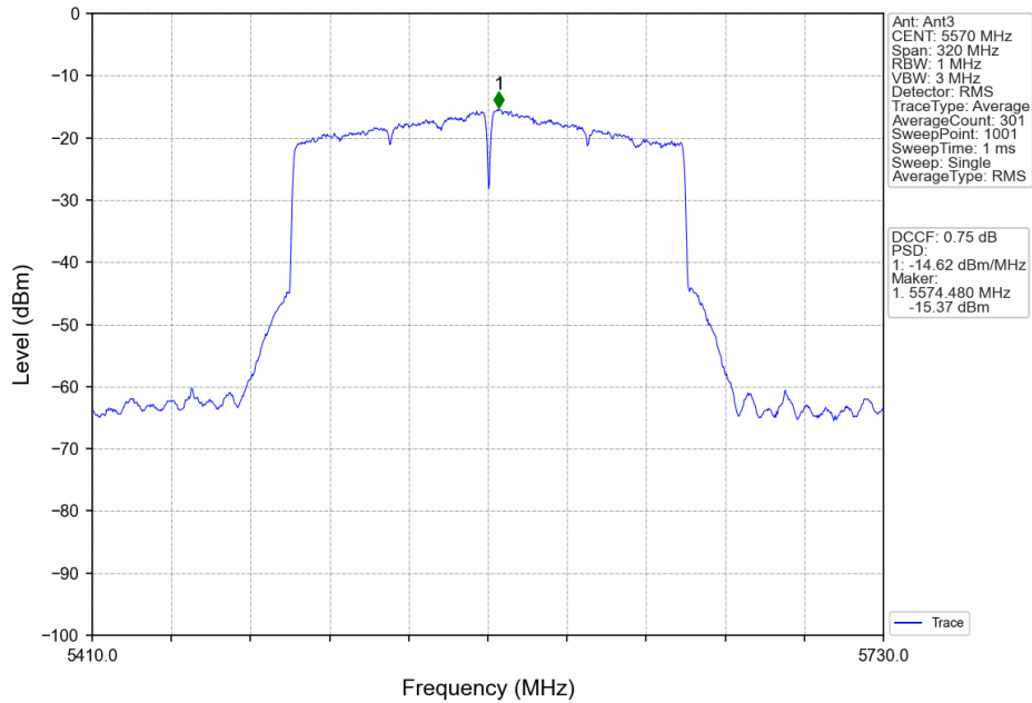
802.11ax(HEW160)_MCH_5570MHz_2xRU996_Left_MIMO_NTNV
