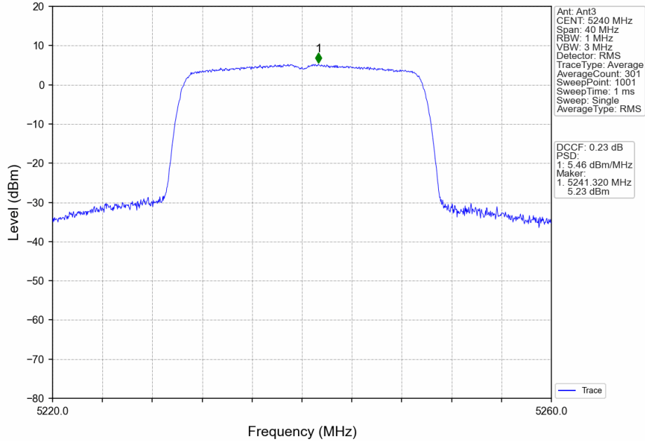
802.11ax(HEW20)_HCH_5240MHz_RU242_Left_MIMO_NTNV
