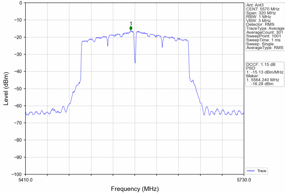
802.11ac(VHT160)_MCH_5570MHz_MIMO_NTNV
