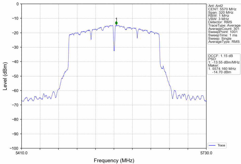
802.11ac(VHT160)_MCH_5570MHz_Ant2_NTNV
