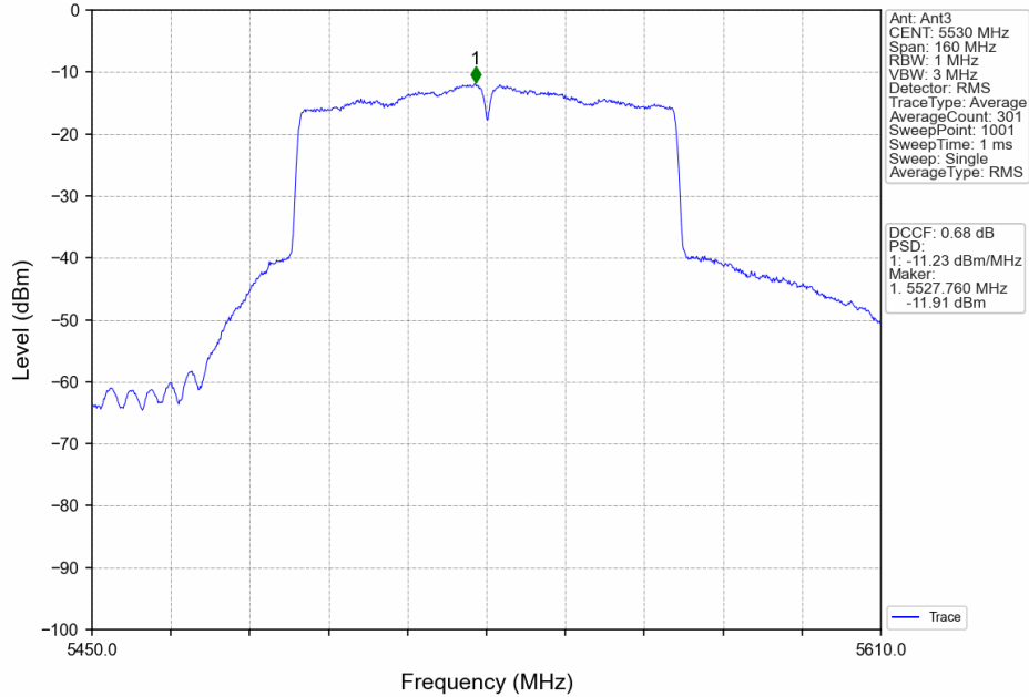
802.11ac(VHT80)_LCH_5530MHz_MIMO_NTNV
