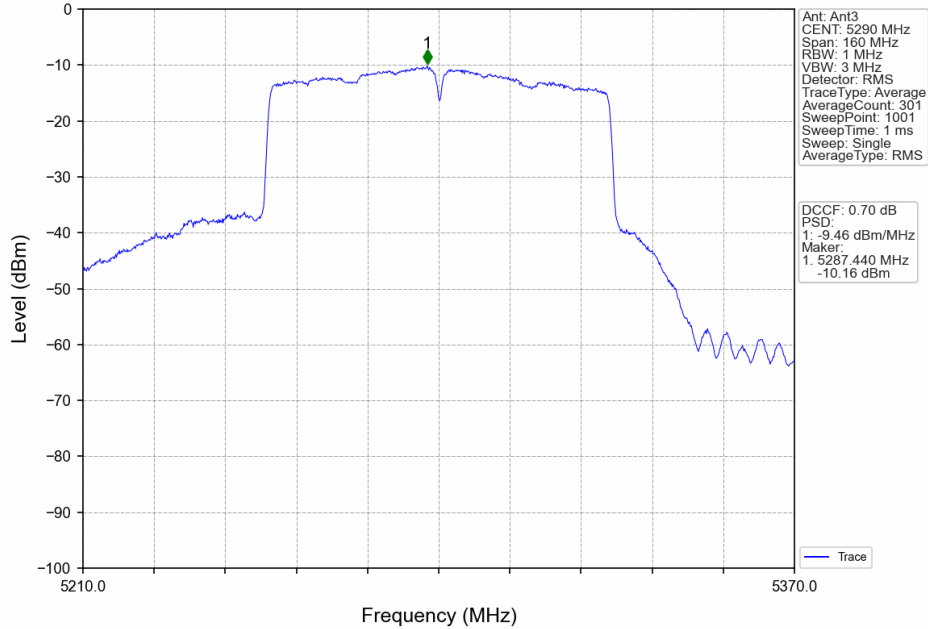
802.11ac(VHT80)_MCH_5290MHz_MIMO_NTNV
