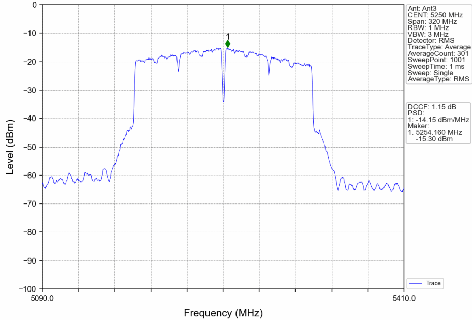
802.11ac(VHT160)_MCH_5250MHz_MIMO_NTNV
