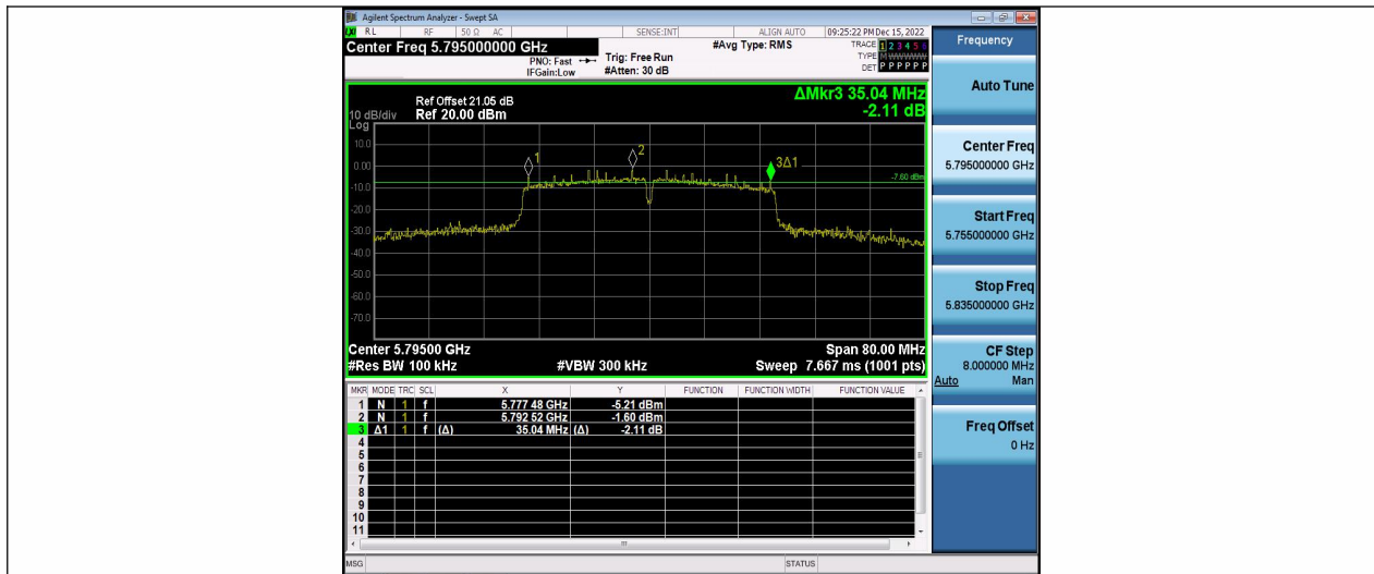
11AC40MIMO Ant2 5795
