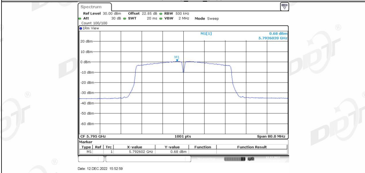
11N40MIMO Ant2 5795
