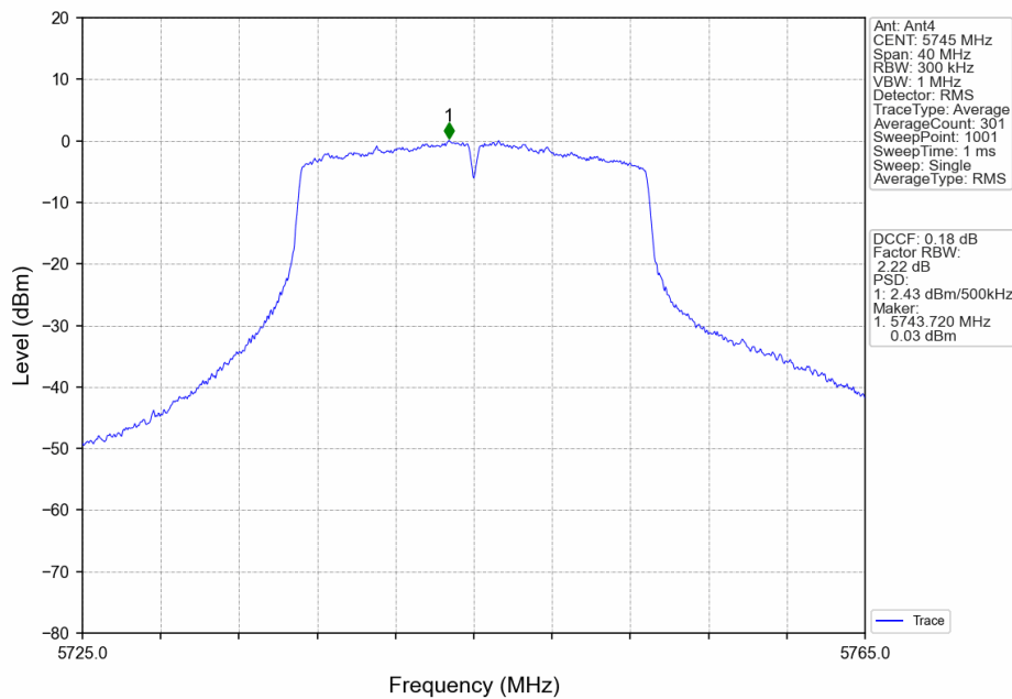
802.11ac(VHT20)_LCH_5745MHz_Ant4_NTNV
