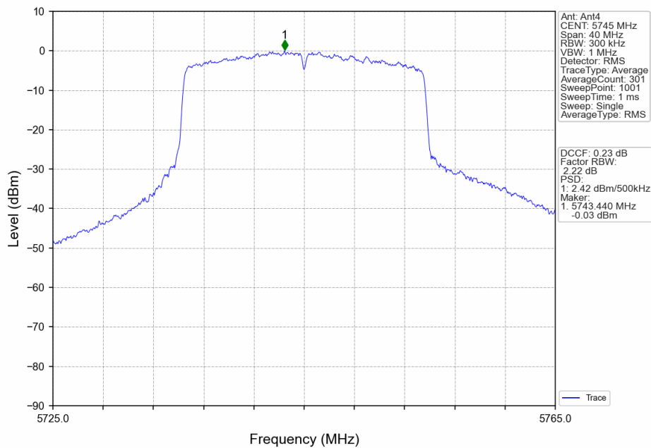
802.11ax(HEW20)_LCH_5745MHz_RU242_Left_Ant4_NTNV
