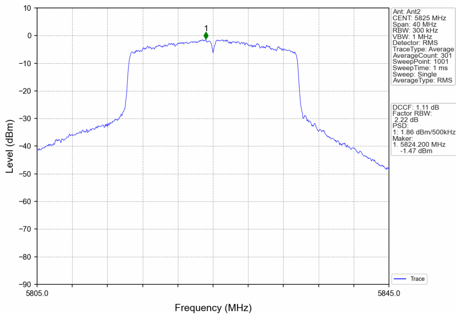
802.11ax(HEW20)_HCH_5825MHz_RU242_Left_Ant2_NTNV
