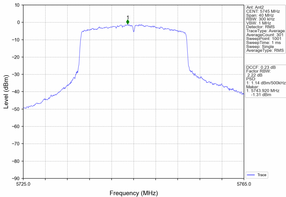
802.11ax(HEW20)_LCH_5745MHz_RU242_Left_Ant2_NTNV
