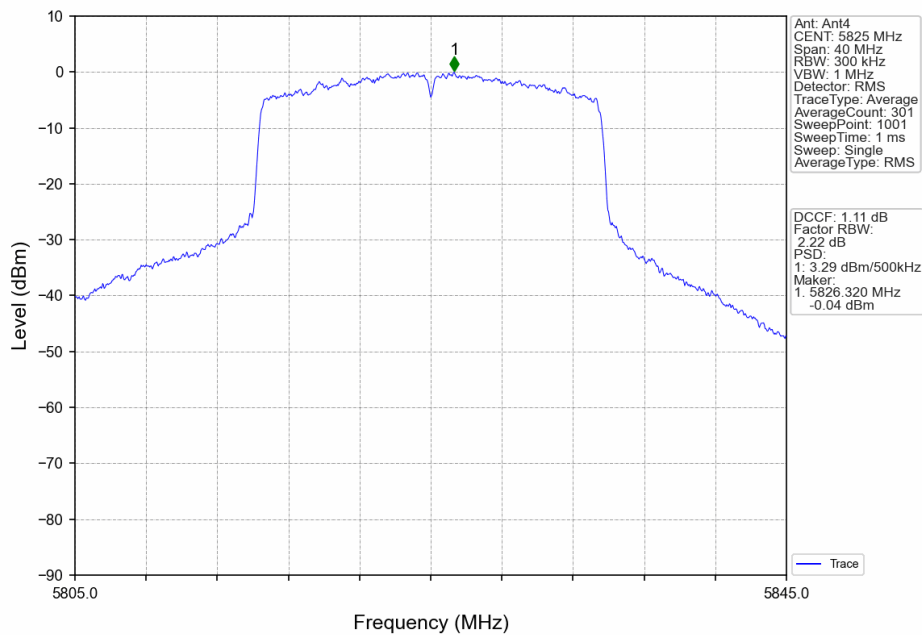
802.11ax(HEW20)_HCH_5825MHz_RU242_Left_Ant4_NTNV
