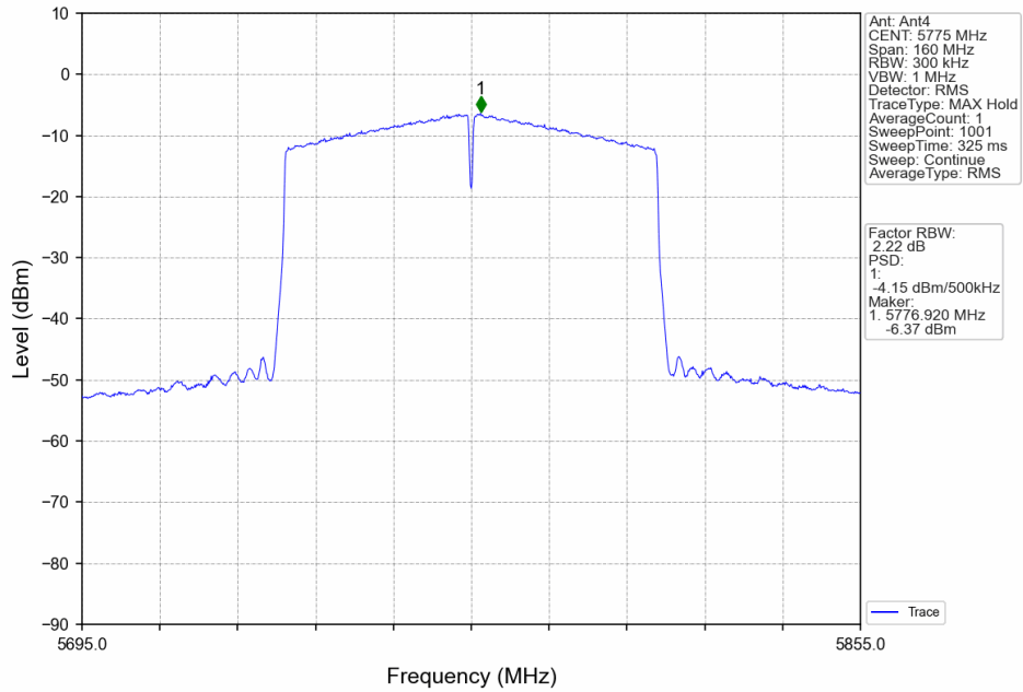
802.11ac(VHT80)_MCH_5775MHz_MIMO_NTNV
