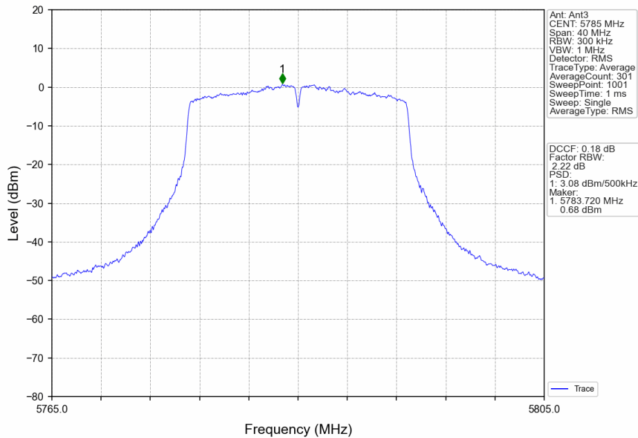
802.11ac(VHT20)_MCH_5785MHz_Ant3_NTNV
