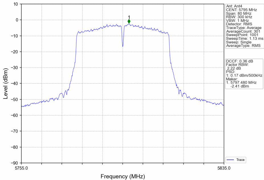
802.11ac(VHT40)_HCH_5795MHz_Ant4_NTNV
