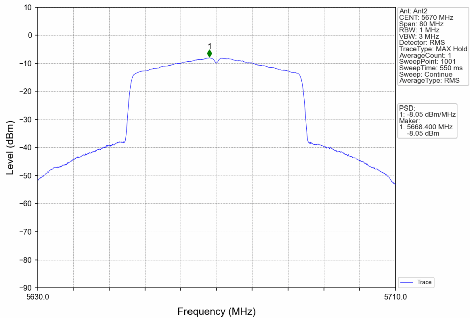
802.11ax(HEW40)_HCH_5670MHz_RU484_Left_Ant2_NTNV
