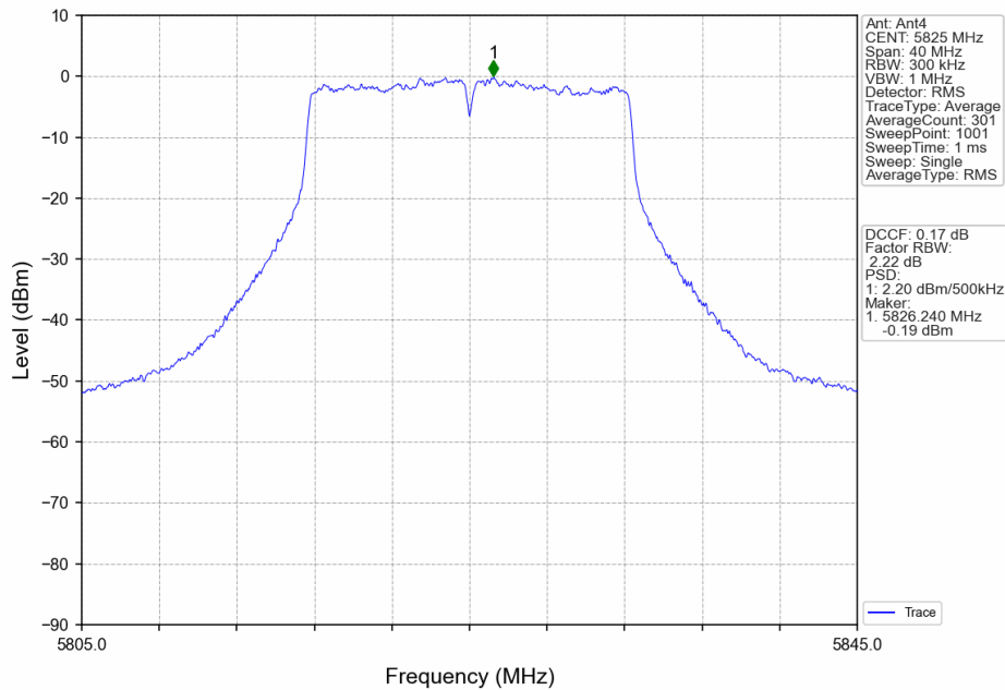
802.11a_HCH_5825MHz_Ant4_NTNV
