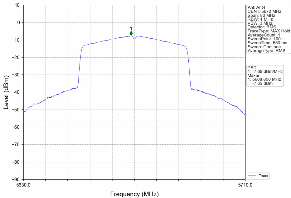
802.11ax(HEW40)_HCH_5670MHz_RU484_Left_Ant4_NTNV
