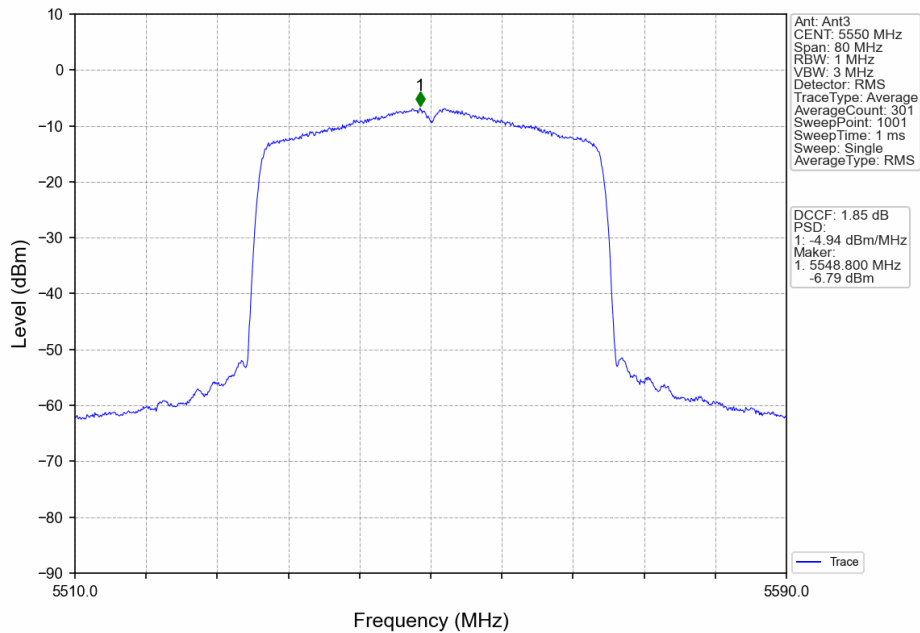
802.11ax(HEW40)_MCH_5550MHz_RU484_Left_Ant3_NTNV
