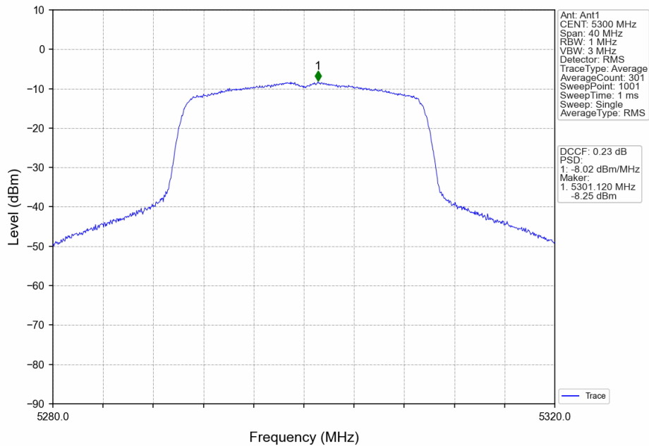
802.11ax(HEW20)_MCH_5300MHz_RU242_Left_Ant1_NTNV
