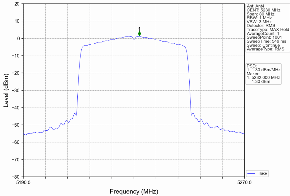
802.11ax(HEW40)_HCH_5230MHz_RU484_Left_MIMO_NTNV
