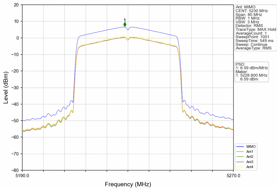
802.11ax(HEW40)_HCH_5230MHz_RU484_Left_MIMO_NTNV
