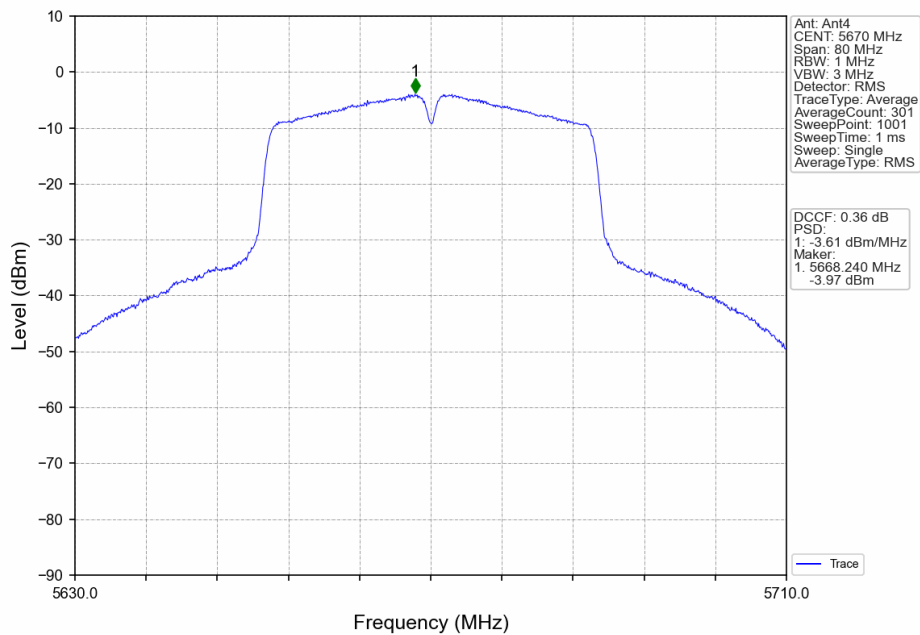
802.11ac(VHT40)_HCH_5670MHz_Ant4_NTNV
