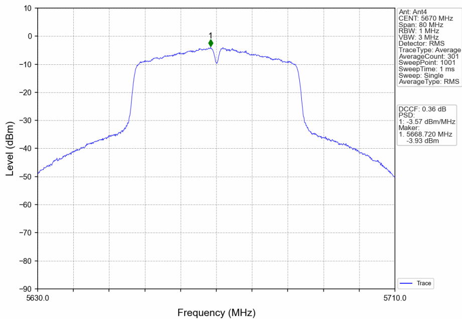
802.11n(HT40)_HCH_5670MHz_Ant4_NTNV
