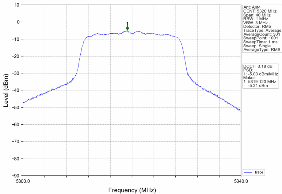
802.11ac(VHT20)_HCH_5320MHz_Ant4_NTNV
