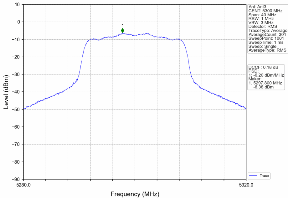
802.11ac(VHT20)_MCH_5300MHz_Ant3_NTNV
