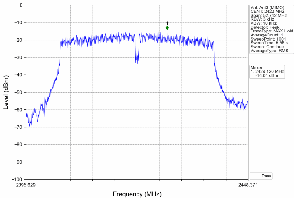
802.11ac(VHT40)_LCH_2422MHz_Ant3 (MIMO)_NTNV
