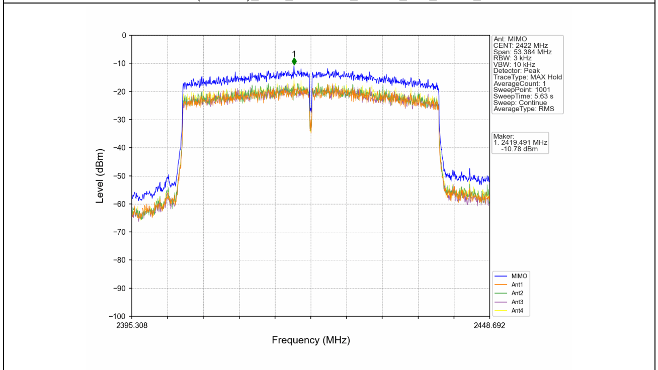
802.11ax(HEW40)_LCH_2422MHz_RU484_Left_MIMO_NTNV
