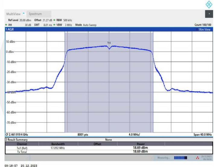
11G_Ant4_2462
