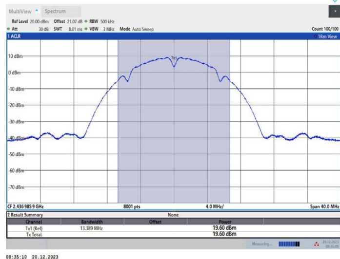
11B_Ant3_2437
