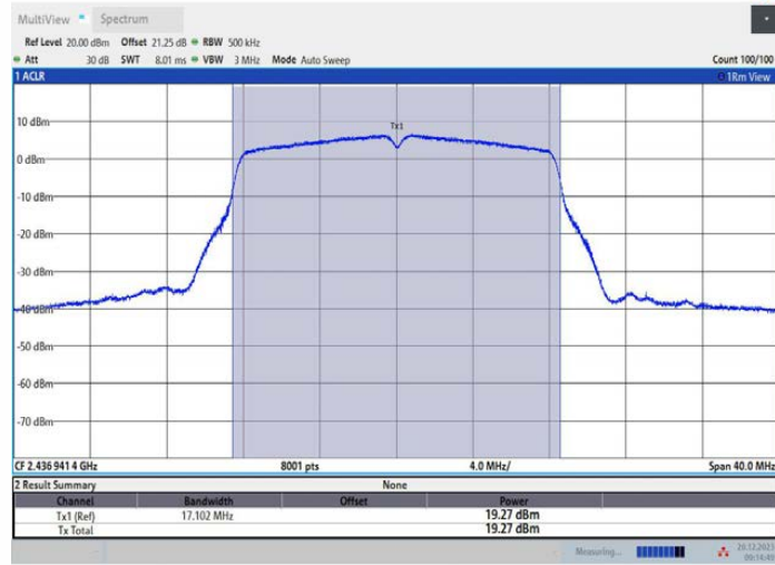
11G_Ant4_2437
