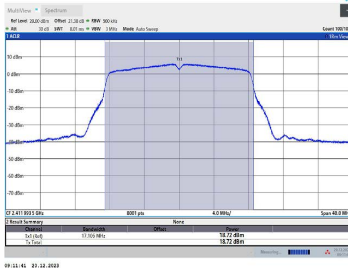
11G_Ant4_2412
