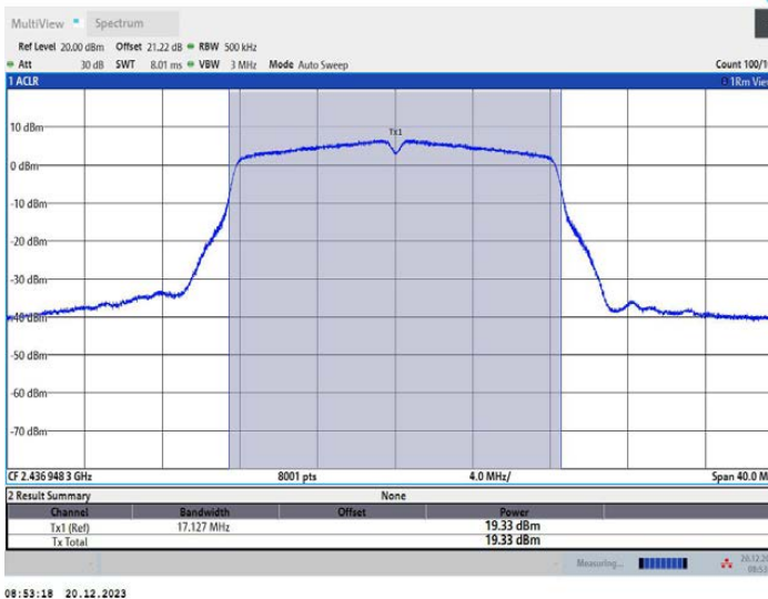
11G_Ant3_2437
