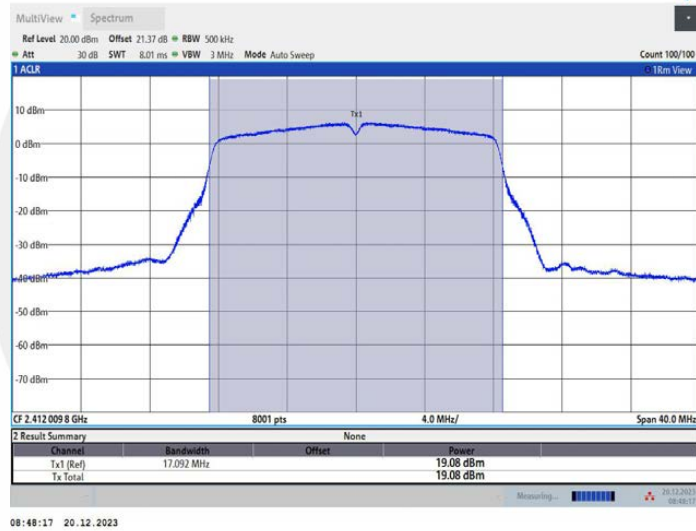
11G_Ant3_2412
