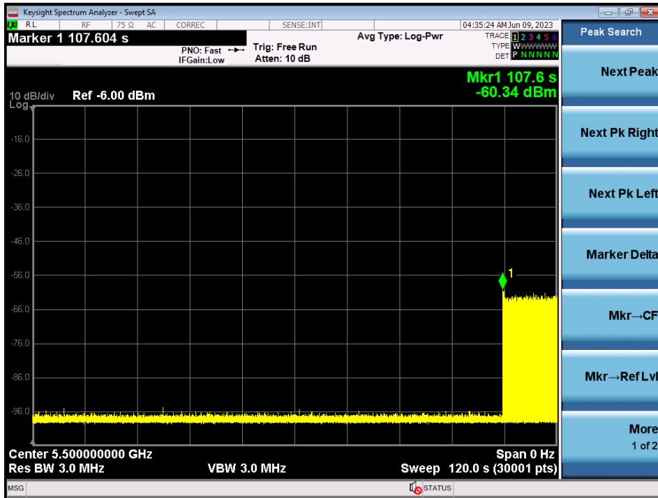
power-on cycle(5500MHz)
