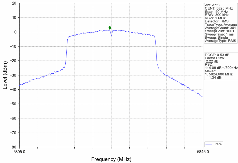
802.11ax(HEW20)_HCH_5825MHz_RU242_Left_MIMO_NTNV
