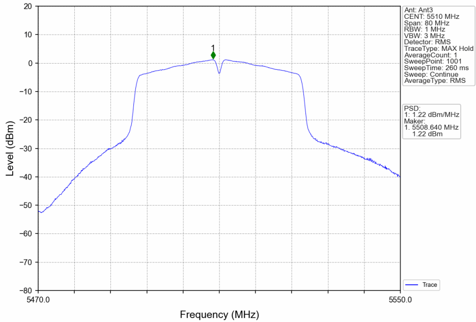
802.11ac(VHT40)_LCH_5510MHz_MIMO_NTNV
