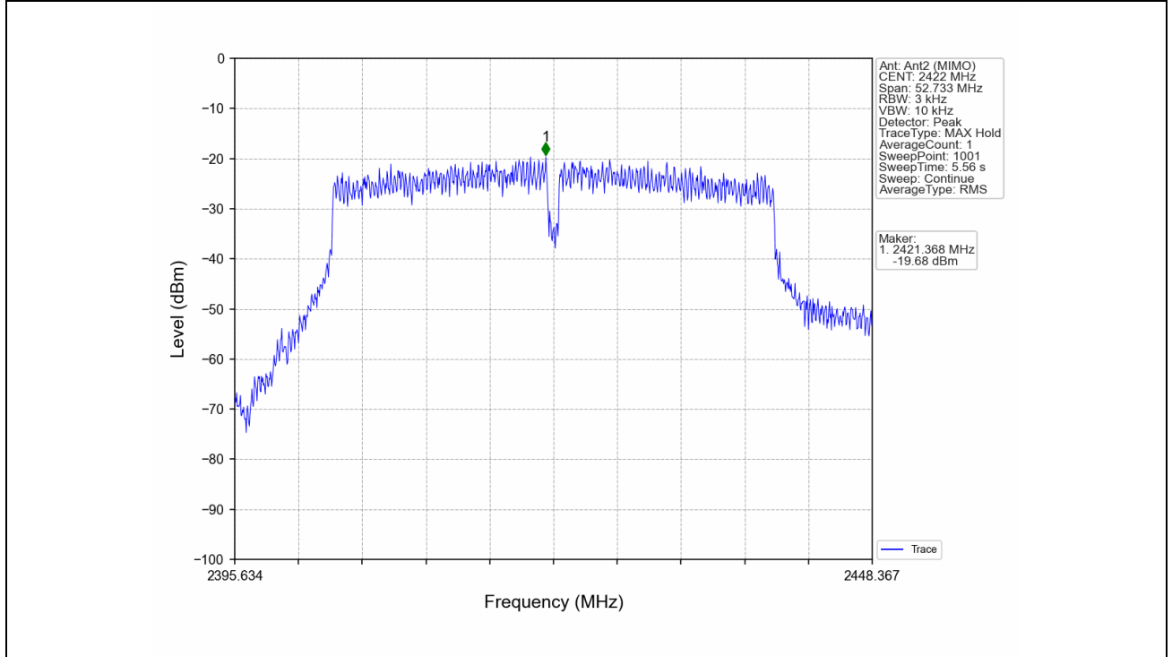
802.11ac(VHT40)_LCH_2422MHz_MIMO_NTNV
