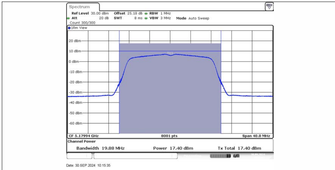
11A_Ant2_5180
