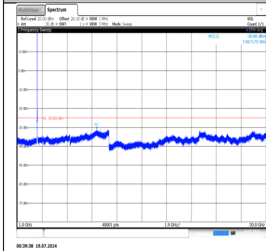
Band7-20MHz-QPSK-20850-1RB#99- 30~1000-PASS
