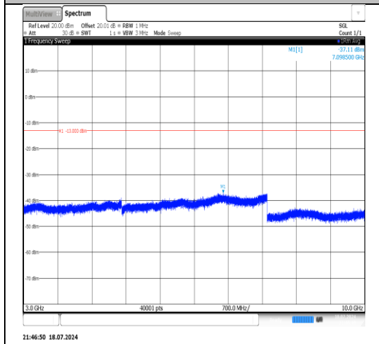
Band5-10MHz-QPSK-20450-50RB#0- 1000~3000-PASS
