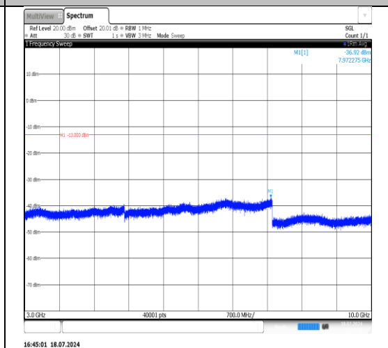
Band5-3MHz-QPSK-20635-1RB#14-1000~3000-PASS
