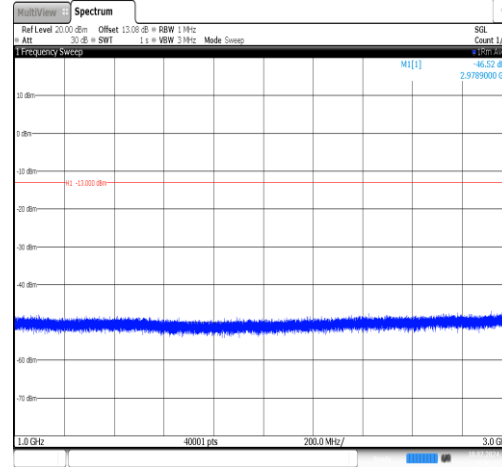
Band5-1.4MHz-QPSK-20407-1RB#5- 1000~3000-PASS
