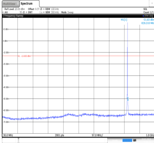
Band5-1.4MHz-QPSK-20407-1RB#5- 30~1000-PASS
