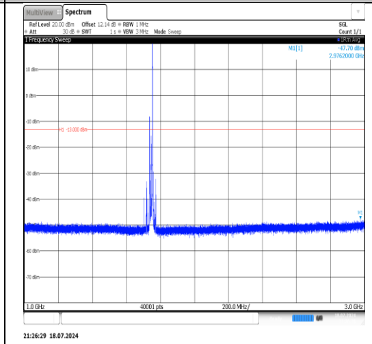
Band4-20MHz-16QAM-20300-1RB#99-1000~3000-PASS
