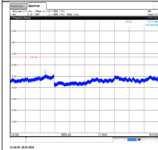
Band4-20MHz-16QAM-20300-1RB#99-3000~20000-PASS
