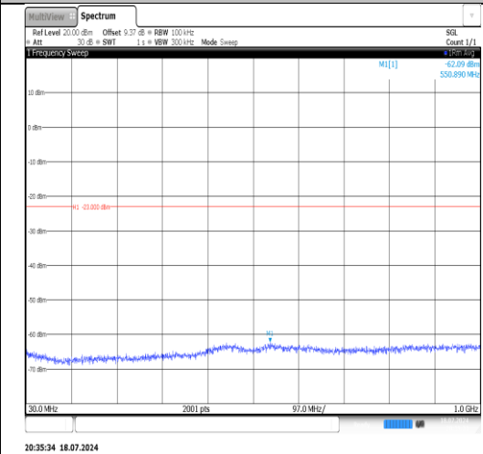
Band4-10MHz-16QAM-20000-1RB#0- 3000~20000-PASS
