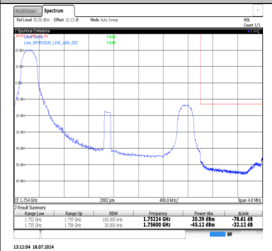
Band4-3MHz-QPSK-20385-1RB#14-PASS
