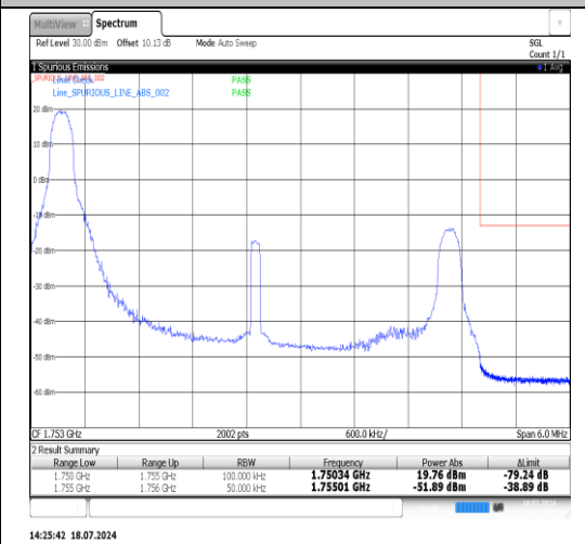
Band4-5MHz-16QAM-20375-1RB#24-PASS
