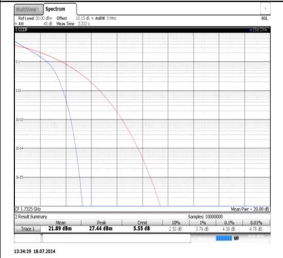
Band4-3MHz-QPSK-20385-15RB#0-PASS
