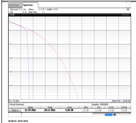
Band4-10MHz-16QAM-20000-1RB#0-PASS
