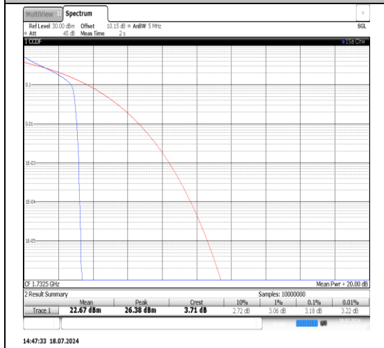
Band4-5MHz-QPSK-20375-1RB#0-PASS
