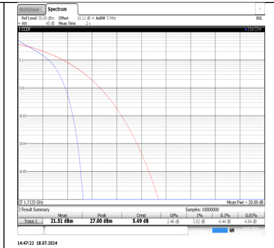
Band4-5MHz-QPSK-20175-25RB#0-PASS
