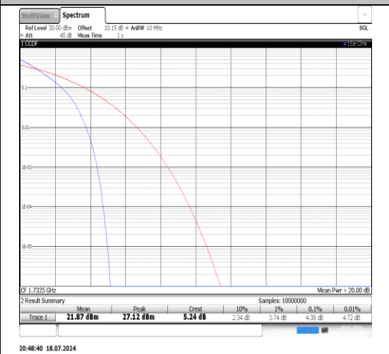
Band4-10MHz-QPSK-20350-50RB#0-PASS
