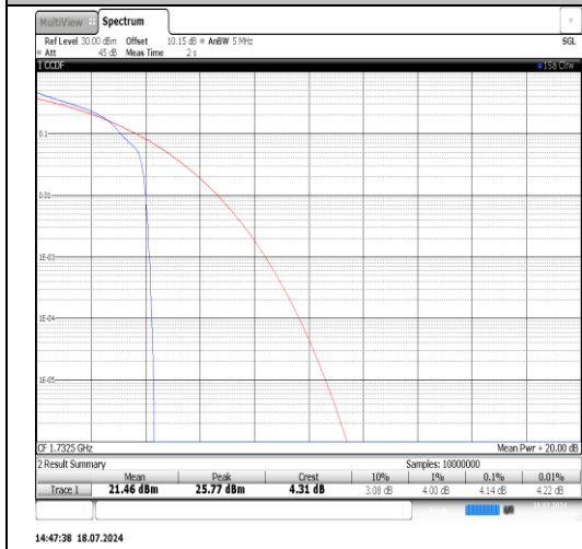
Band4-5MHz-16QAM-20375-1RB#0-PASS
