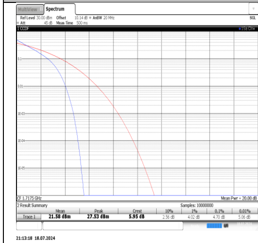
Band4-15MHz-QPSK-20175-75RB#0-PASS
