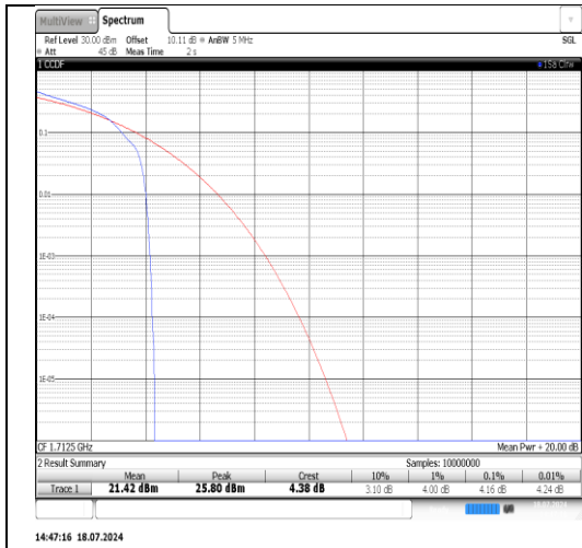
Band4-5MHz-16QAM-20175-1RB#0-PASS
