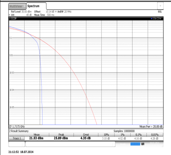
Band4-15MHz-16QAM-20325-1RB#0-PASS
