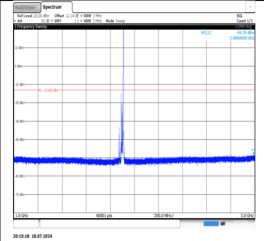
Band2-20MHz-16QAM-19100-1RB#99-1000~3000-PASS
