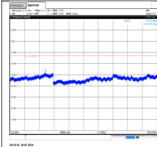
Band2-20MHz-16QAM-19100-1RB#99-3000~20000-PASS
