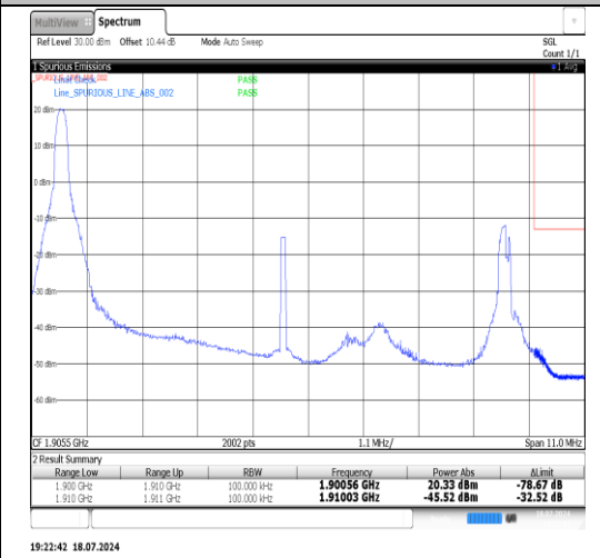
Band2-10MHz-QPSK-19150-1RB#49-PASS
