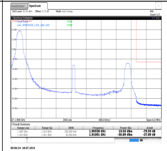
Band2-5MHz-16QAM-19175-1RB#24-PASS
