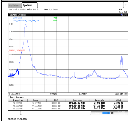
Band12-10MHz-QPSK-23060-1RB#49-PASS
