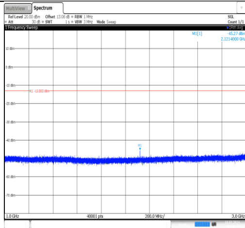
Band12-1.4MHz-QPSK-23095-1RB#0- 1000~3000-PASS
