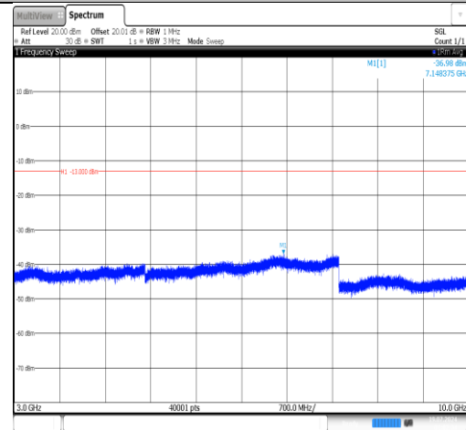
Band12-1.4MHz-QPSK-23095-1RB#0- 3000~10000-PASS
