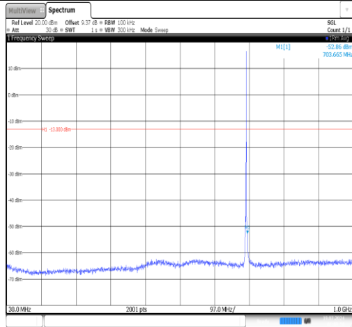
Band12-1.4MHz-QPSK-23017-1RB#5- 30~1000-PASS
