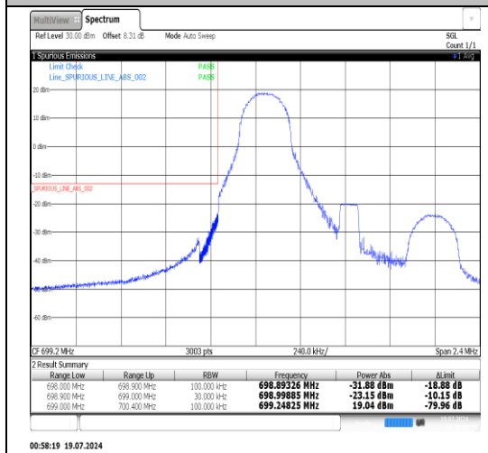
Band12-1.4MHz-16QAM-23017-1RB#5-PASS
