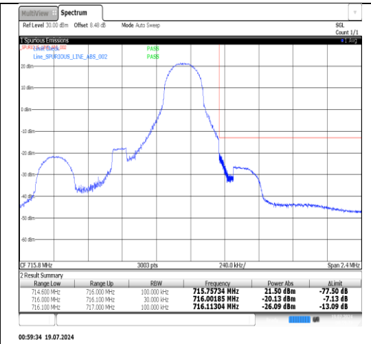
Band12-1.4MHz-16QAM-23017-6RB#0-PASS
