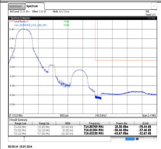
Band12-1.4MHz-16QAM-23173-1RB#5-PASS
