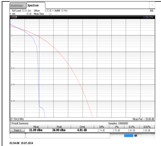
Band12-10MHz-QPSK-23095-1RB#0-PASS
