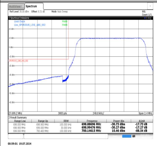
Band12-1.4MHz-16QAM-23173-1RB#0-PASS
