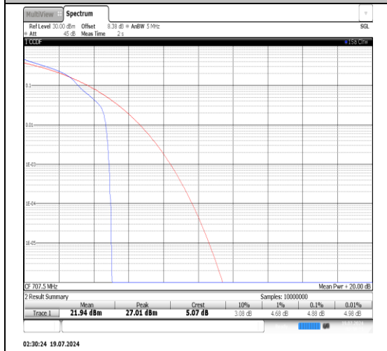
Band12-5MHz-16QAM-23155-1RB#0-PASS
