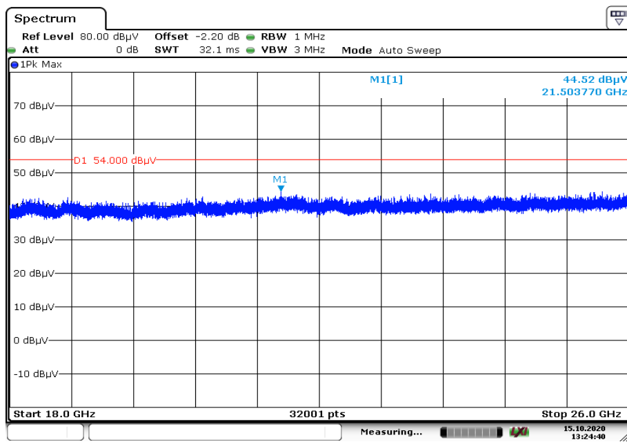
Plot 10: 18 GHz to 26 GHz, TX mode, 2402 MHz, vertical & horizontal polarization, 2 Msps
