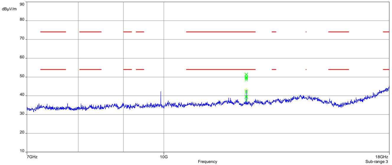
Plot 7: 7 GHz to 18 GHz, TX mode, 2480 MHz, vertical & horizontal polarization, 1 Msps
