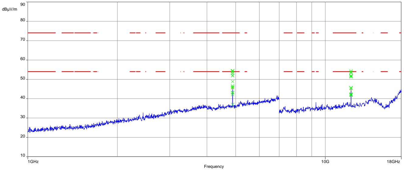
Plot 11: 1 GHz to 18 GHz, TX mode, 2440 MHz, vertical & horizontal polarization, 2 Msps
