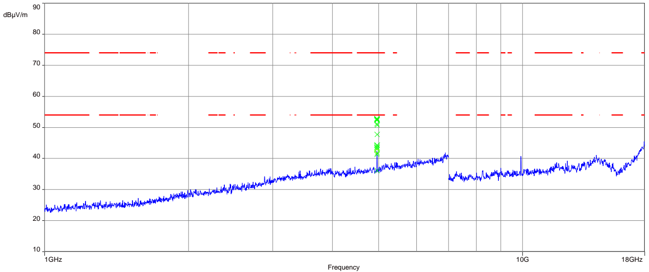
Plot 13: 1 GHz to 18 GHz, TX mode, 2480 MHz, vertical & horizontal polarization, 2 Msps
