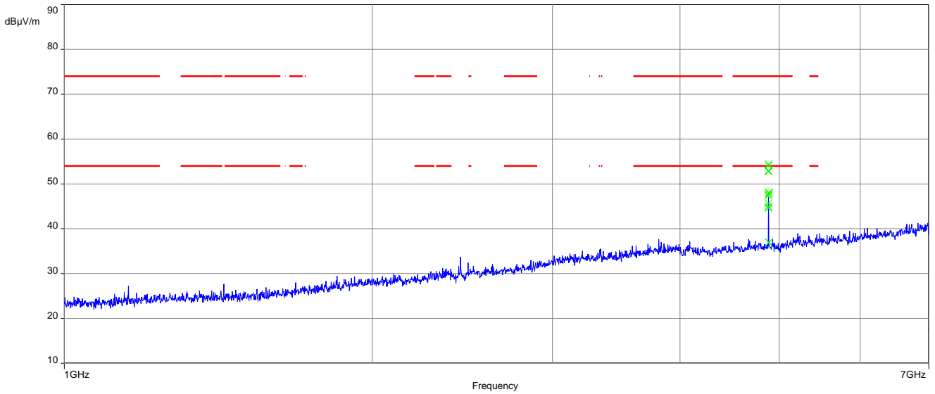
Plot 3: 1 GHz to 7 GHz, TX mode, 2440 MHz, vertical & horizontal polarization, 1 Msps
