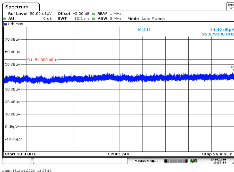
Plot 14: 18 GHz to 26 GHz, TX mode, 2480 MHz, vertical & horizontal polarization, 2 Msps
