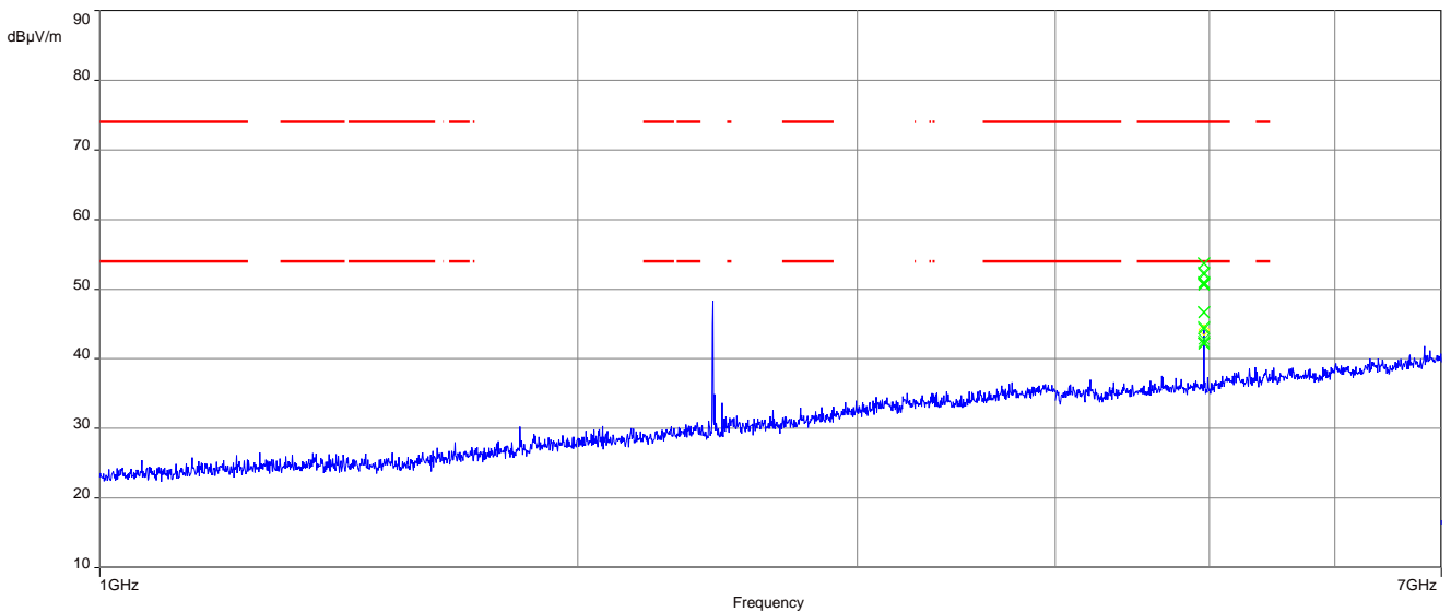
Plot 6: 1 GHz to 7 GHz, TX mode, 2480 MHz, vertical & horizontal polarization, 1 Msps
