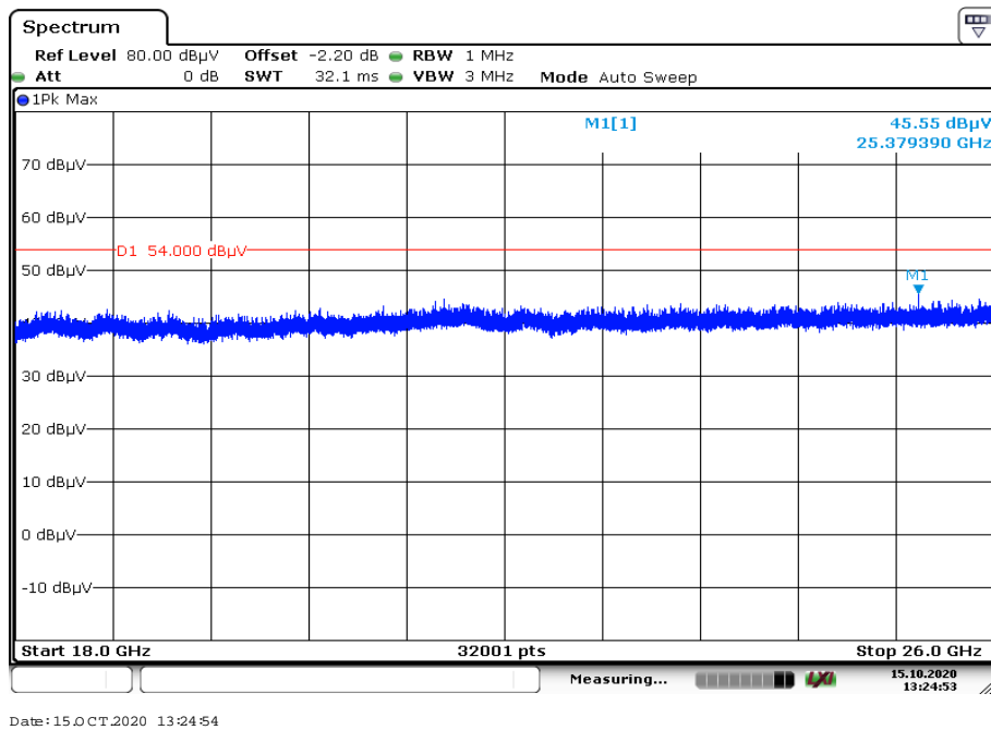
Plot 12: 18 GHz to 26 GHz, TX mode, 2440 MHz, vertical & horizontal polarization, 2 Msps
