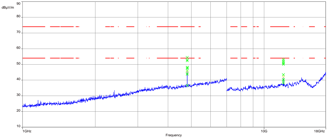
Plot 9: 1 GHz to 18 GHz, TX mode, 2402 MHz, vertical & horizontal polarization, 2 Msps
