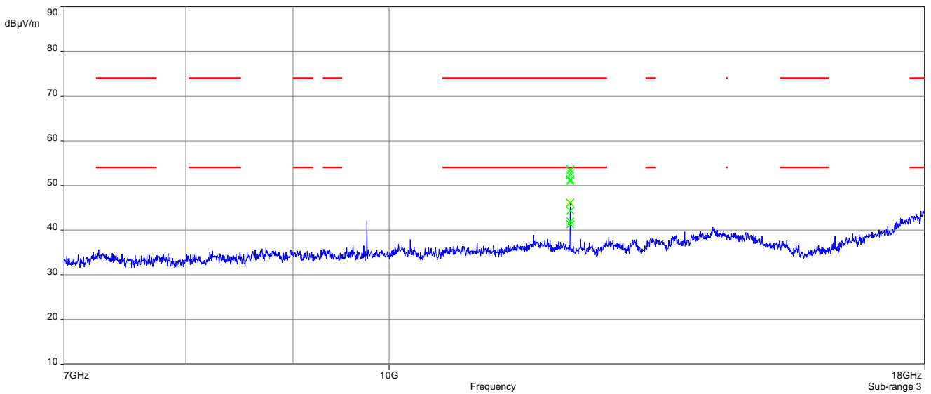
Plot 4: 7 GHz to 18 GHz, TX mode, 2440 MHz, vertical & horizontal polarization, 1 Msps
