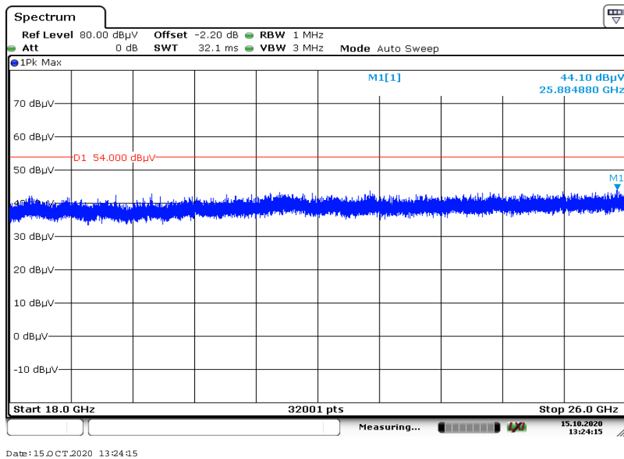
Plot 8: 18 GHz to 26 GHz, TX mode, 2480 MHz, vertical & horizontal polarization, 1 Msps
