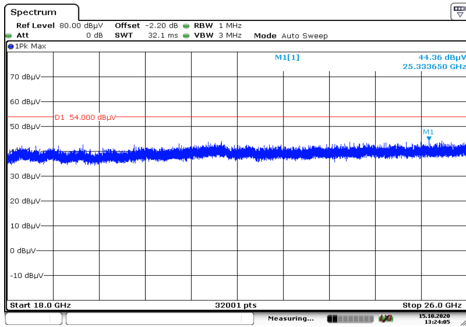
Plot 5: 18 GHz to 26 GHz, TX mode, 2440 MHz, vertical & horizontal polarization, 1 Msps
