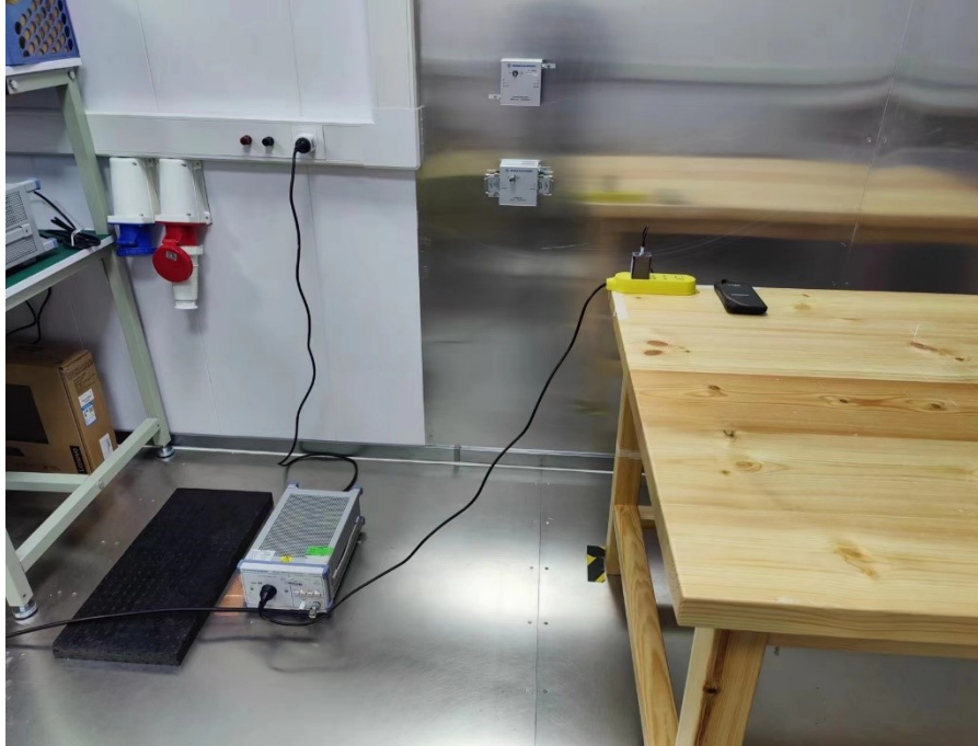
Conducted Emissions (0.15-30MHz)
