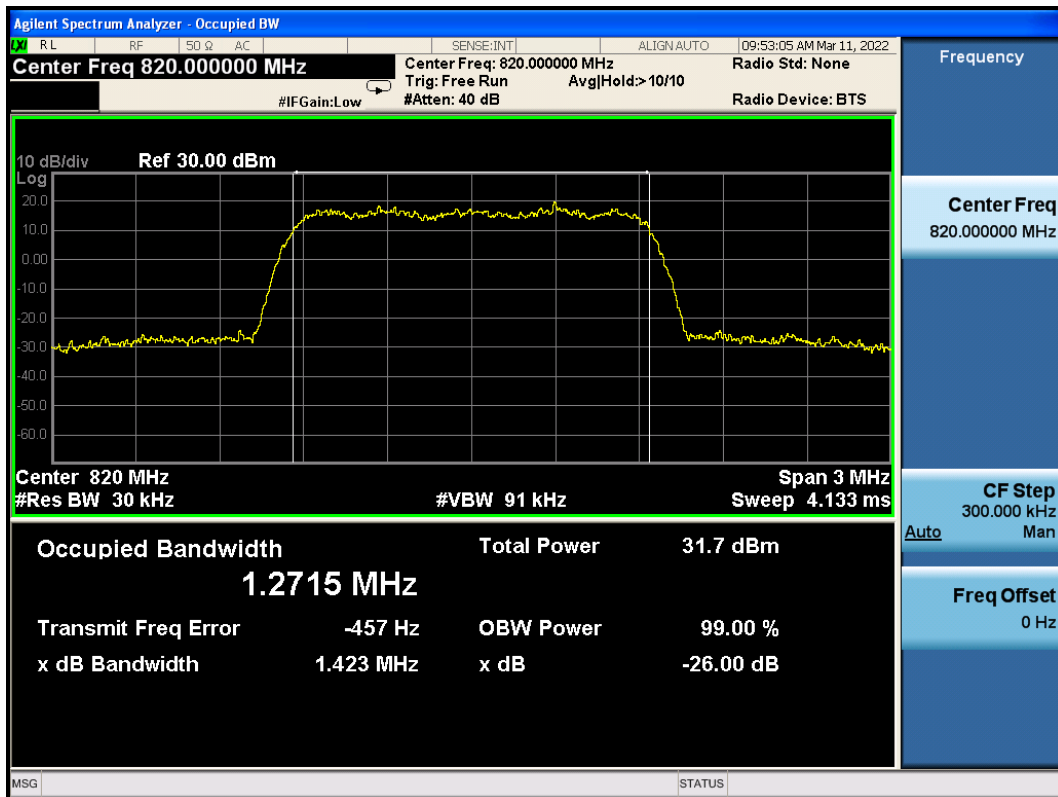
CDMA2000 BC10 1xRTT Channel=670
