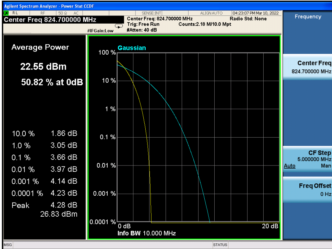
CDMA2000 BC0 1xRTT Channel=1013
