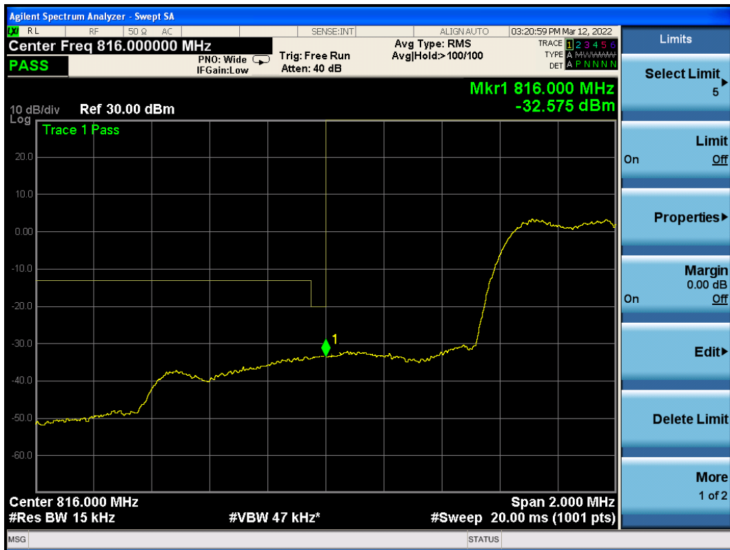
CDMA2000 BC10 1xEV-Do Rel.A Channel=670
