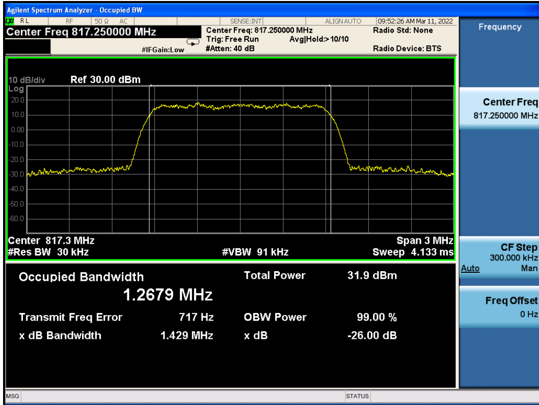
CDMA2000 BC10 1xRTT Channel=560
