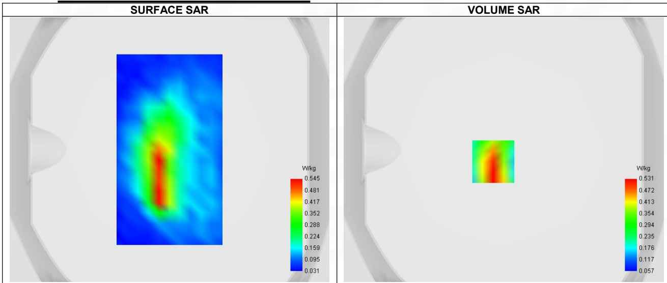
Maximum location: X=-1.00, Y=15.00 ; SAR Peak: 0.98 W/kg
