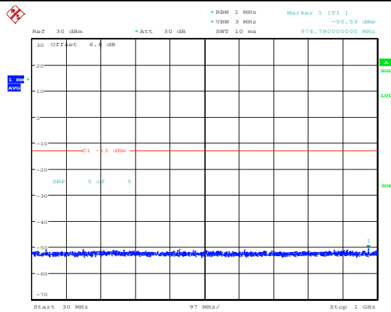
Band25-20MHz-QPSK-26140-1RB#0-Range3:30~1000MHz
