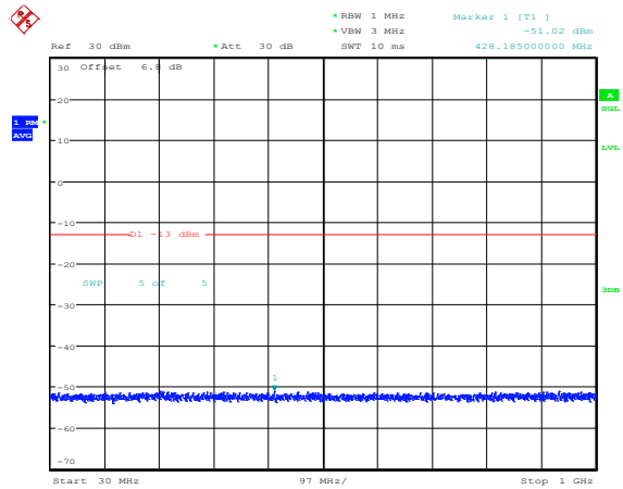
Band25-15MHz-QPSK-26115-1RB#0-Range3:30~1000MHz
