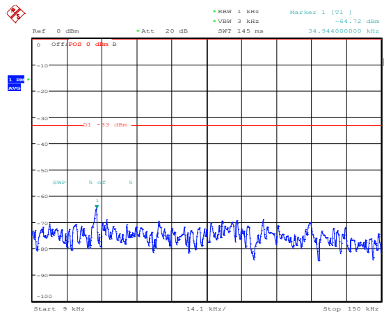
Band25-1.4MHz-16QAM-26683-1RB#0-Range1:0.009~0.15MHz
