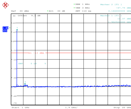
Band25-10MHz-16QAM-26640-1RB#0-Range4:1000~20000MHz
