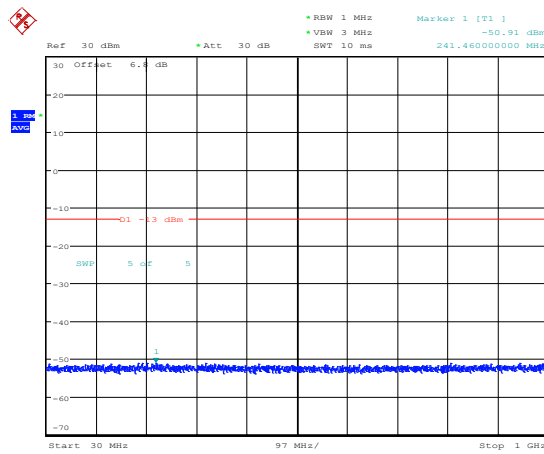
Band25-10MHz-16QAM-26640-1RB#0-Range3:30~1000MHz
