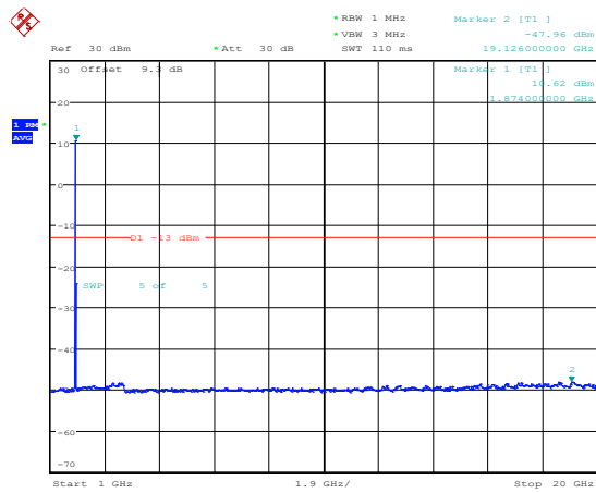
Band25-10MHz-16QAM-26365-1RB#0-Range4:1000~20000MHz
