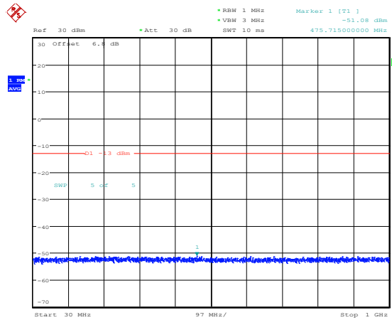
Band25-10MHz-QPSK-26090-1RB#0-Range3:30~1000MHz
