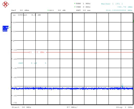
Band25-5MHz-16QAM-26065-1RB#0-Range3:30~1000MHz
