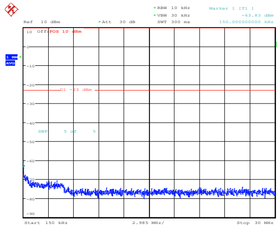
Band25-5MHz-16QAM-26065-1RB#0-Range2:0.15~30MHz
