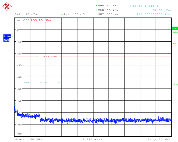
Band25-3MHz-16QAM-26055-1RB#0-Range2:0.15~30MHz
