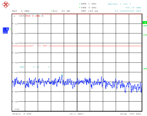
Band25-15MHz-16QAM-26365-1RB#0-Range1:0.009~0.15MHz
