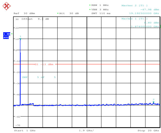
Band25-1.4MHz-16QAM-26365-1RB#0-Range4:1000~20000MHz
