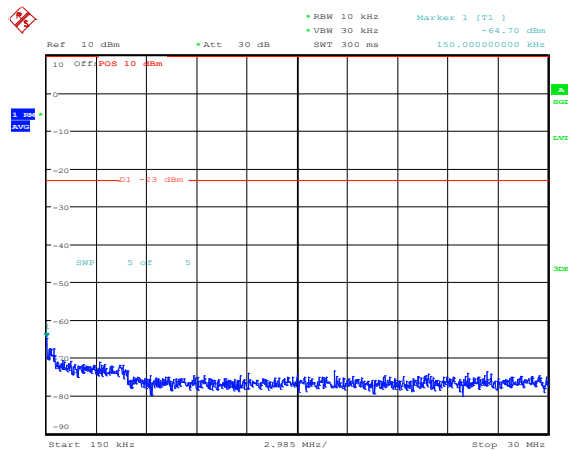
Band25-15MHz-16QAM-26365-1RB#0-Range2:0.15~30MHz
