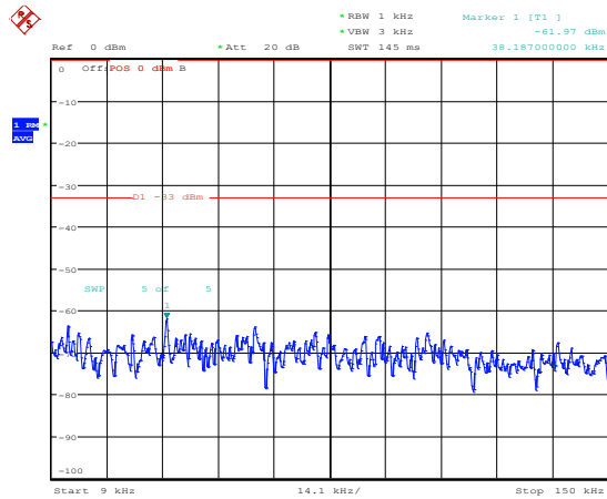
Band25-10MHz-16QAM-26640-1RB#0-Range1:0.009~0.15MHz
