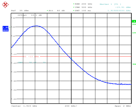
Band25-10MHz-QPSK-26640-1RB#49
