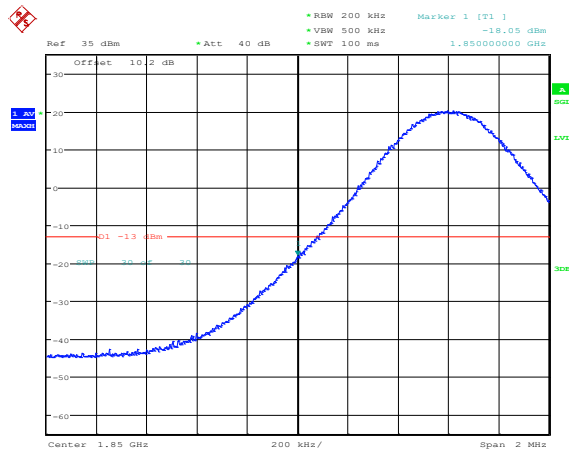
Band25-10MHz-16QAM-26090-1RB#0
