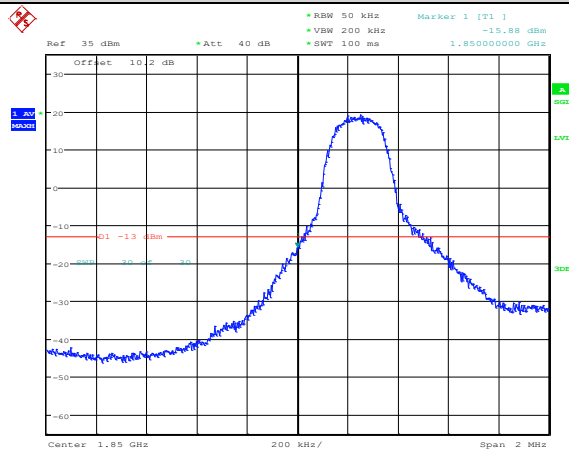
Band25-3MHz-QPSK-26055-1RB#0
