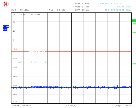
Band25-1.4MHz-QPSK-26047-1RB#0-Range3:30~1000MHz
