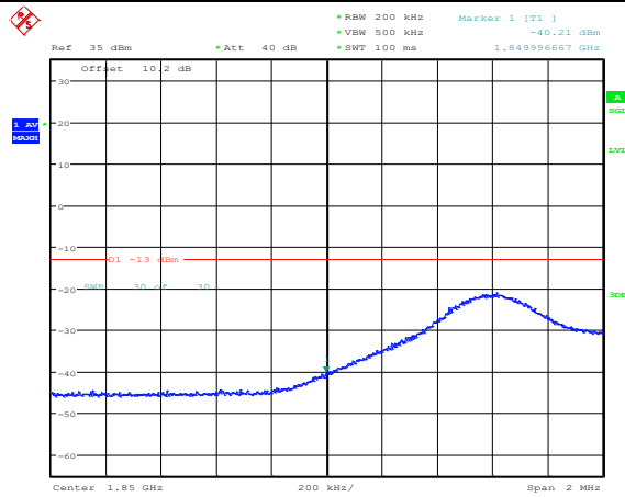
Band25-10MHz-QPSK-26090-1RB#49
