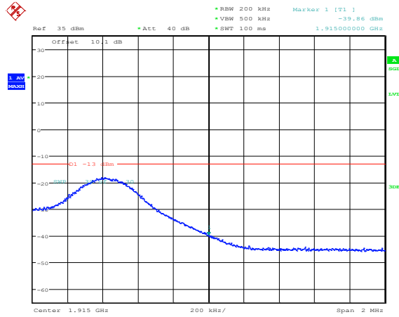
Band25-10MHz-16QAM-26640-1RB#0
