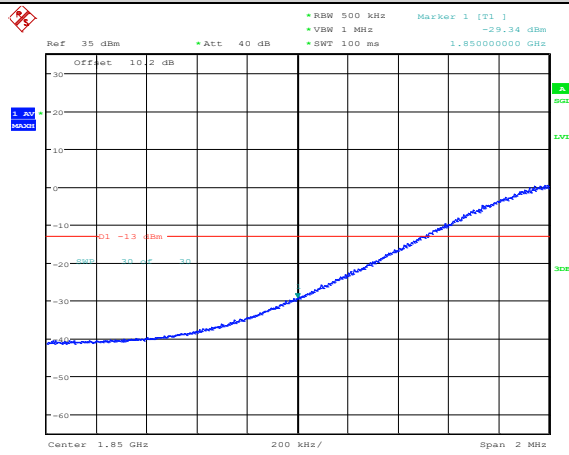
Band25-20MHz-QPSK-26140-100RB#0
