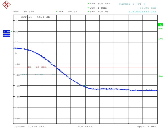
Band25-15MHz-16QAM-26115-1RB#0
