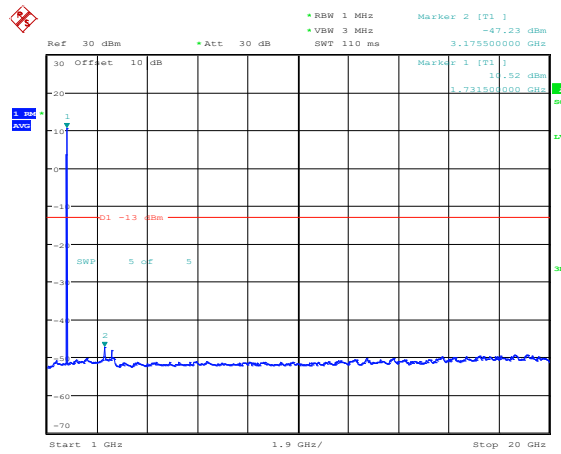
Band4-3MHz-16QAM-20175-1RB#0-Range4:1000~20000MHz
