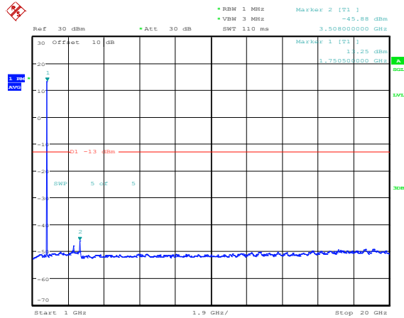
Band4-1.4MHz-16QAM-20393-1RB#0-Range4:1000~20000MHz
