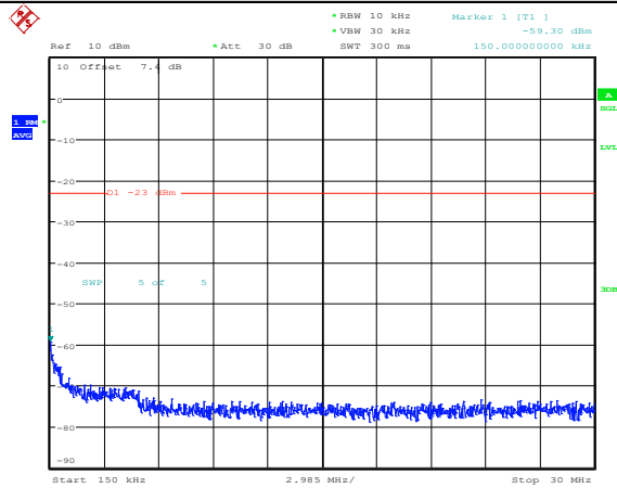
Band4-3MHz-16QAM-20175-1RB#0-Range2:0.15~30MHz
