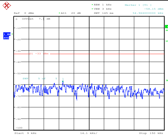
Band4-1.4MHz-16QAM-20393-1RB#0-Range1:0.009~0.15MHz
