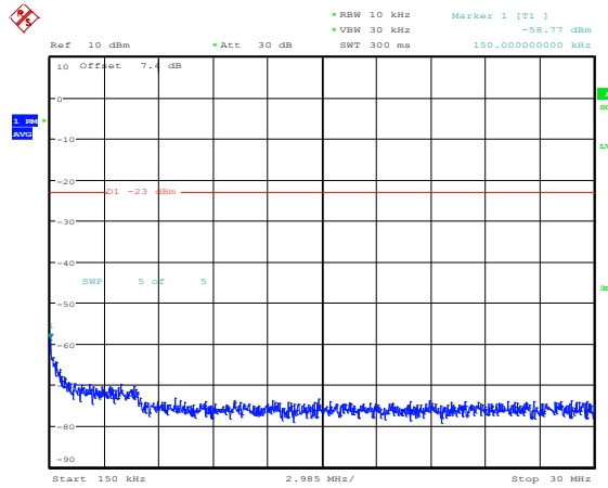
Band4-1.4MHz-16QAM-19957-1RB#0-Range2:0.15~30MHz
