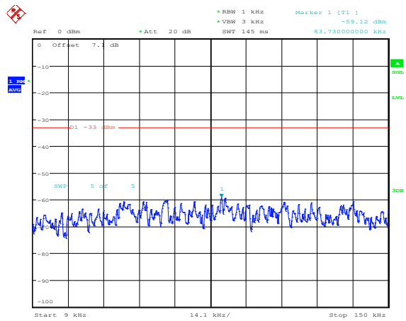
Band4-20MHz-QPSK-20175-1RB#0-Range1:0.009~0.15MHz
