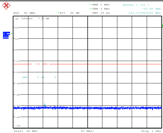
Band4-5MHz-16QAM-19975-1RB#0-Range3:30~1000MHz
