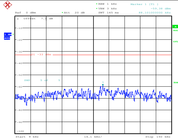
Band4-1.4MHz-QPSK-19957-1RB#0-Range1:0.009~0.15MHz
