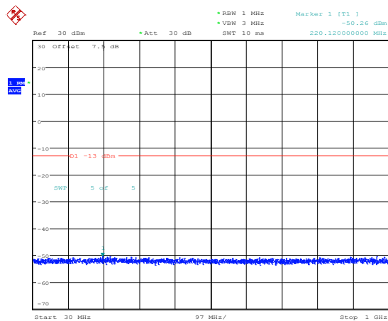
Band4-10MHz-16QAM-20000-1RB#0-Range3:30~1000MHz
