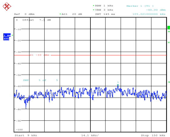
Band4-20MHz-QPSK-20300-1RB#0-Range1:0.009~0.15MHz
