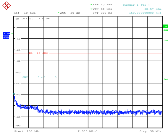
Band4-3MHz-16QAM-19965-1RB#0-Range2:0.15~30MHz
