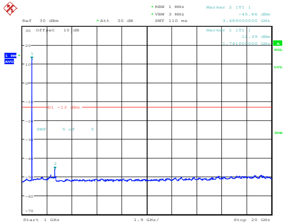
Band4-10MHz-16QAM-20350-1RB#0-Range4:1000~20000MHz
