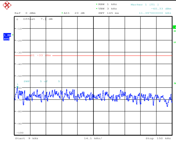
Band4-3MHz-16QAM-20385-1RB#0-Range1:0.009~0.15MHz
