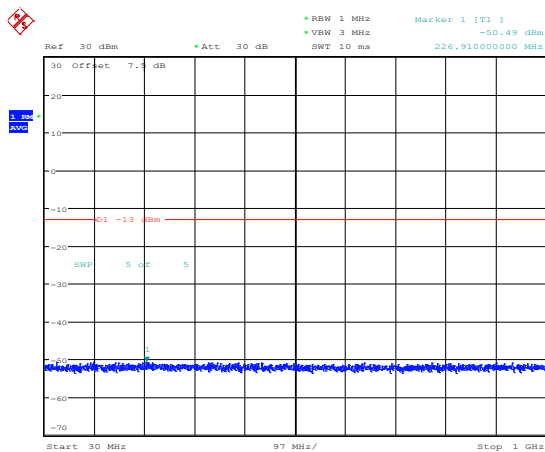
Band4-15MHz-QPSK-20025-1RB#0-Range3:30~1000MHz
