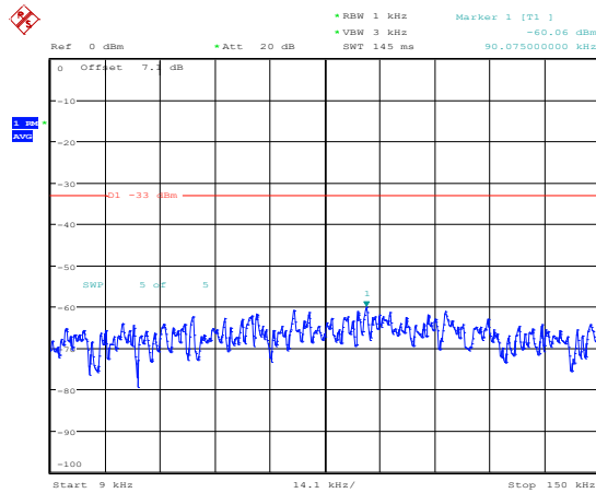
Band4-1.4MHz-QPSK-20175-1RB#0-Range1:0.009~0.15MHz
