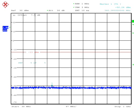
Band4-20MHz-QPSK-20300-1RB#0-Range3:30~1000MHz
