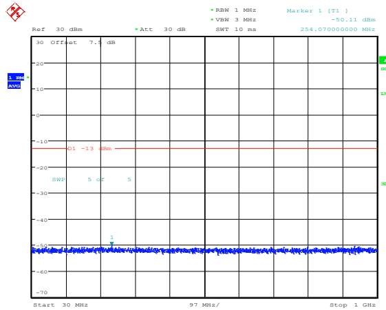
Band4-1.4MHz-16QAM-19957-1RB#0-Range3:30~1000MHz
