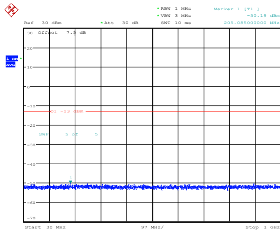
Band4-20MHz-QPSK-20050-1RB#0-Range3:30~1000MHz
