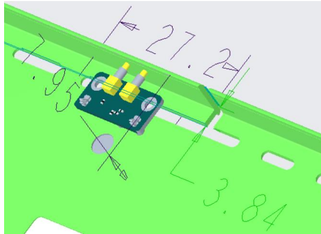
GSM/WDMA/LTE Aux: 27.2*7.95*3.84mm LOOP
