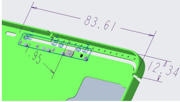
GSM/WDMA/LTE Main: 83.61*7.95*12.34mm LOOP
