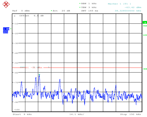
Band41-5MHz-QPSK-40265-1RB#0-Range1:0.009~0.15MHz
