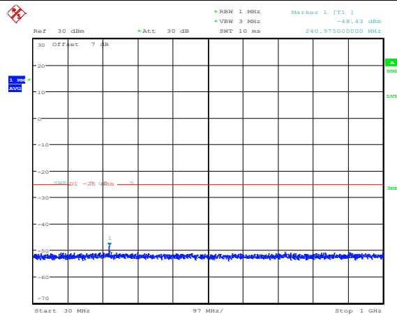
Band41-5MHz-QPSK-40265-1RB#0-Range3:30~1000MHz
