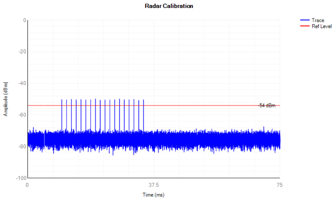
Signal Calibration_802.11a_2A_5260MHz_RadarType0_Trial0
