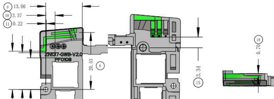
Ant2-GWB: PIFA
